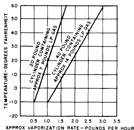
Fig. 7—Vaporization Rate—One-Third Full
