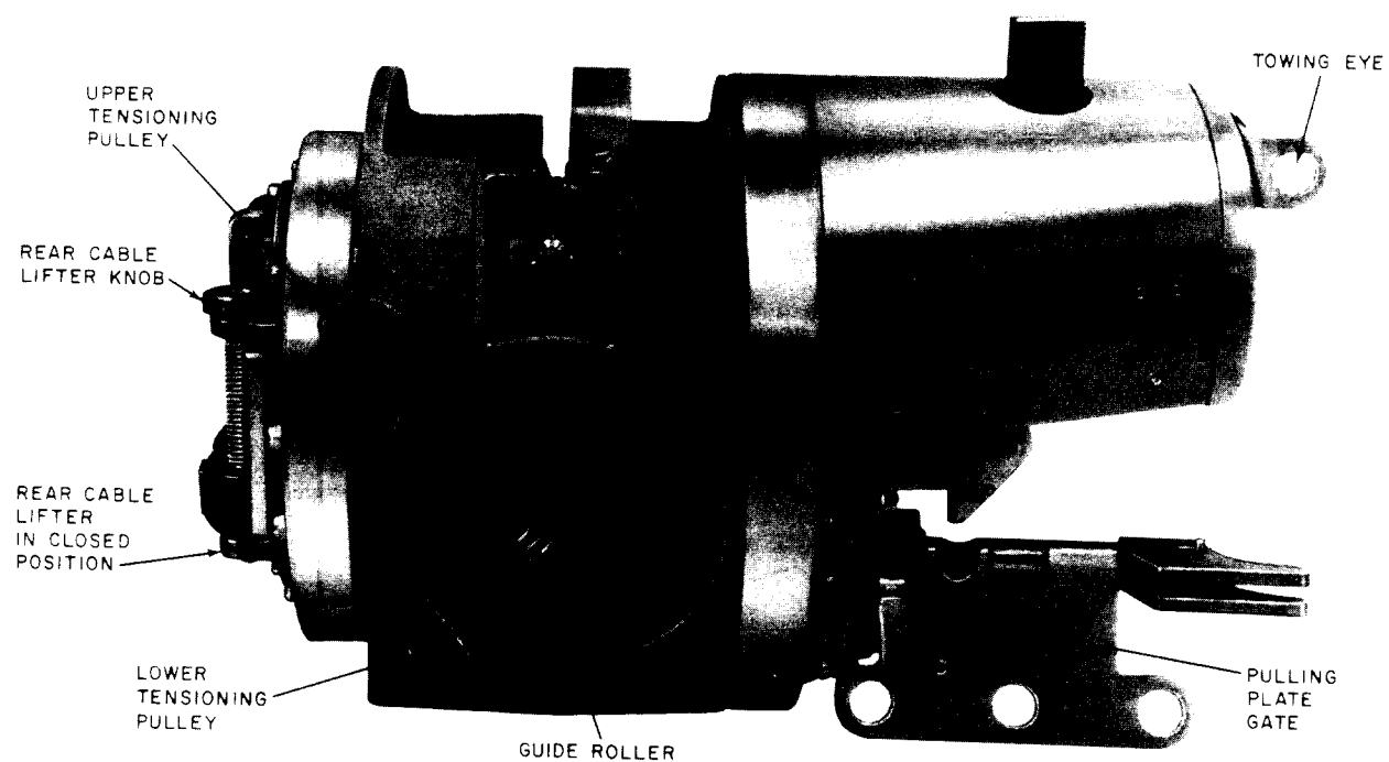
Fig. 2—Left Side of Lasher
