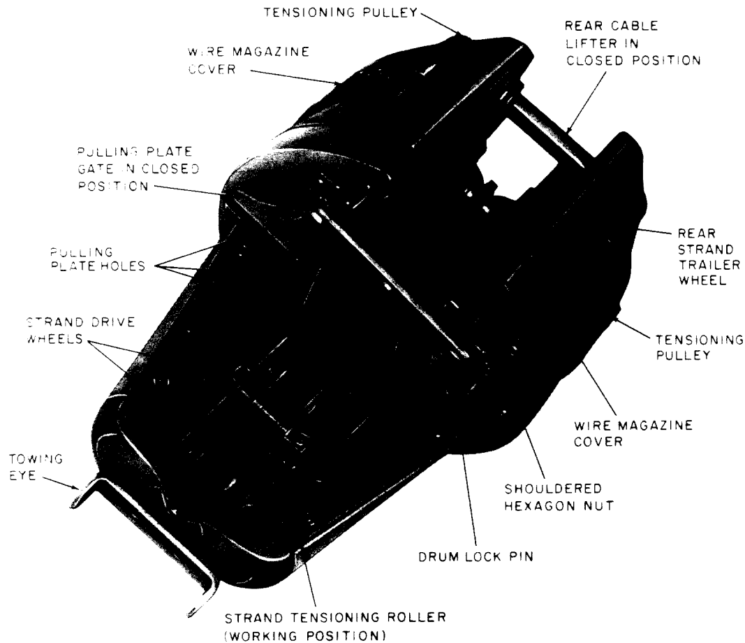
Fig. 3—Under Side of Lasher
