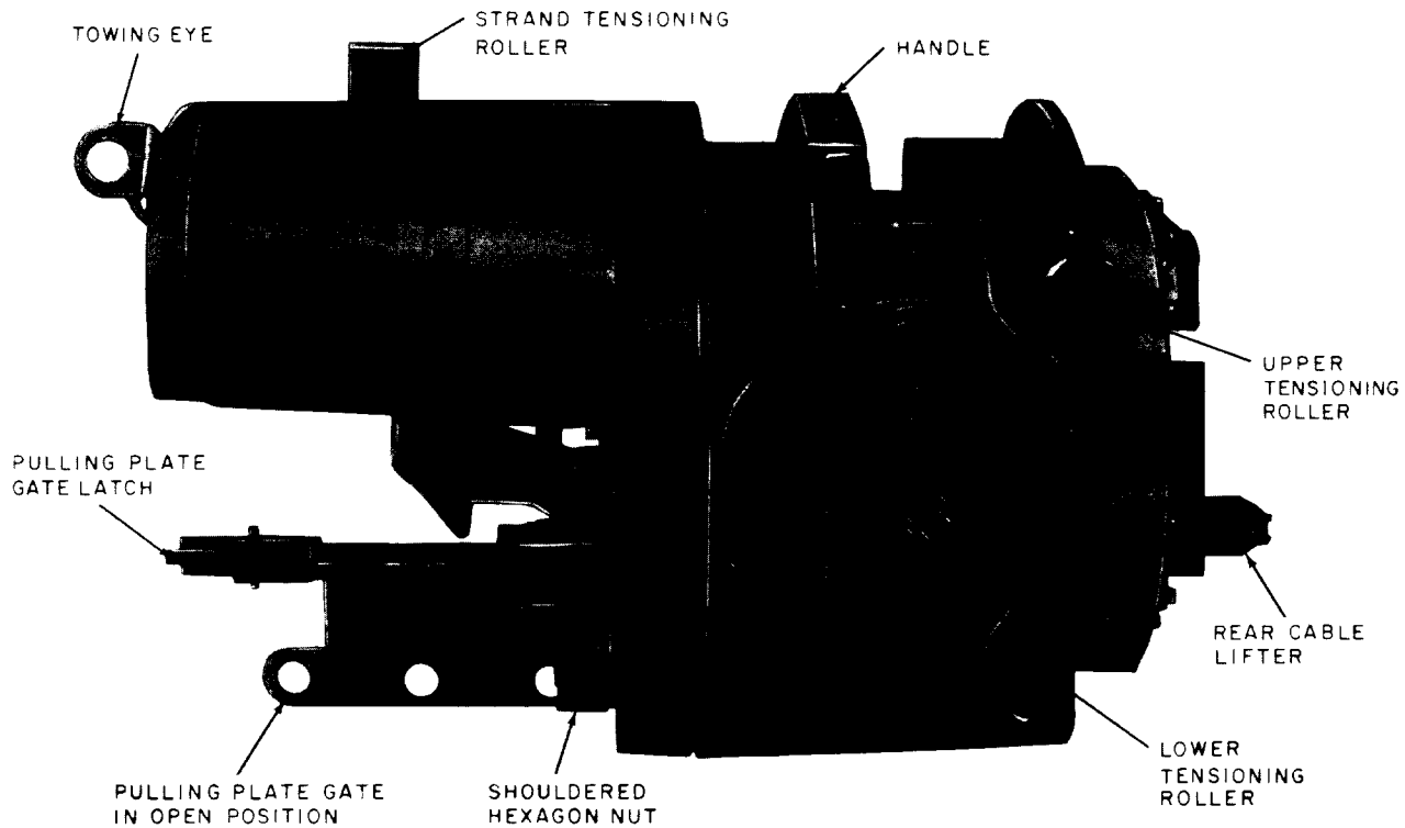
Fig. 1—Right Side of Lasher
