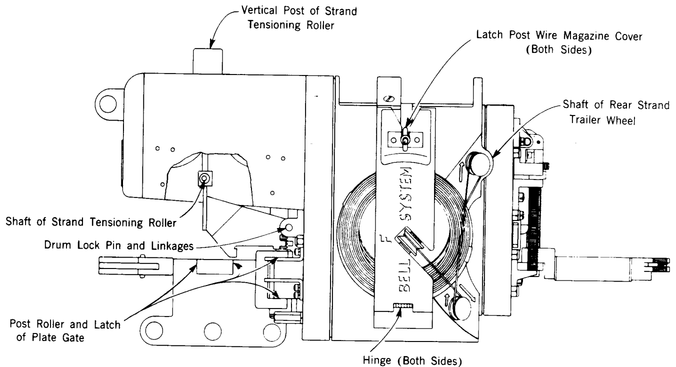
Fig. 8—Side View (Lubrication Chart)
