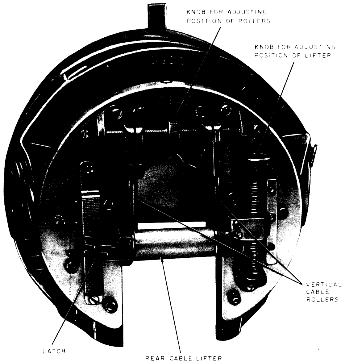
Fig. 4—Rear View of Lasher
