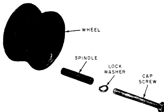
Fig. 10—Plain Wheel
