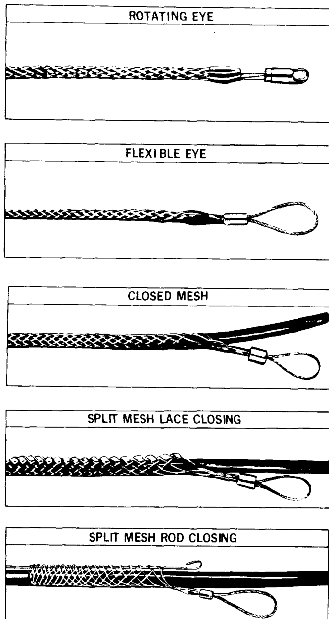
Fig. 1—Typical Pulling Grip Styles (Metallic and Lightguide)
