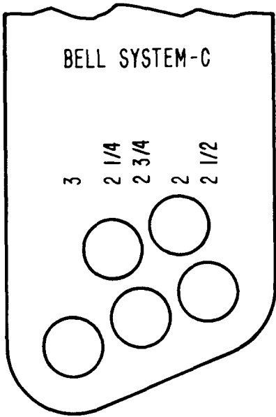
Fig. 2 — Angle Insert Adjustment for C Cable Guide
