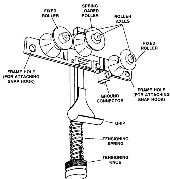
Figure 2 - B Grounding Roller - Early Design
