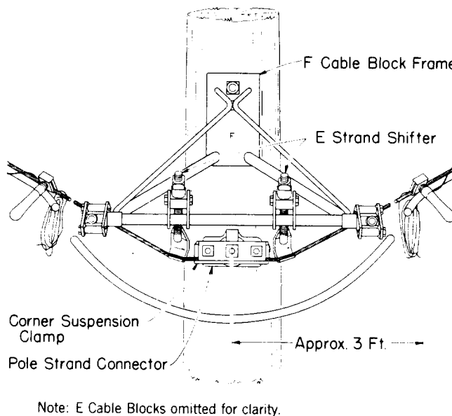
Fig. 18—E Strand Shifter Installed on F Cable Block Frame
