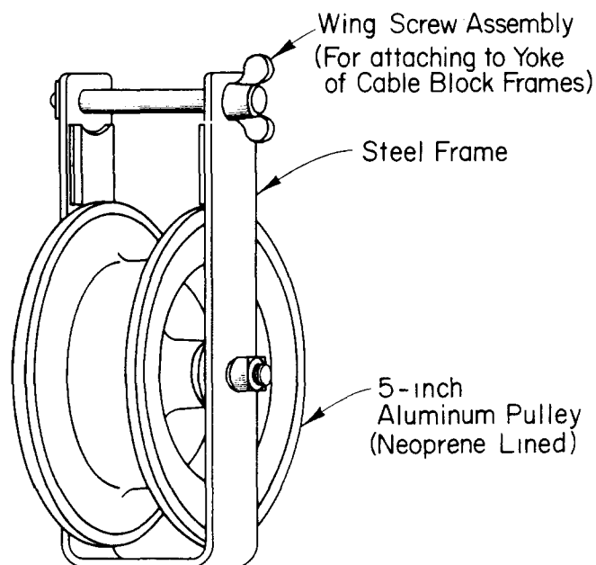
Fig. 1—E Cable Block
