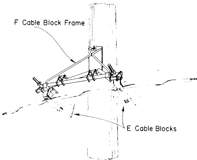
Fig. 12—F Cable Block Frame (With Two E Cable Blocks Installed)
