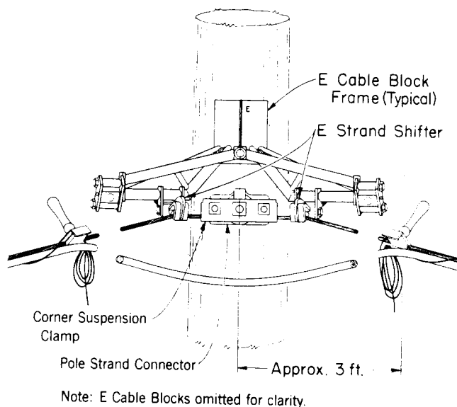
Fig. 17—E Strand Shifter Installed on Typical E Cable Block Frame
