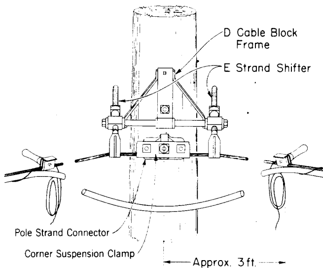
Fig. 16—E Strand Shifter Installed on D Cable Block Frame
