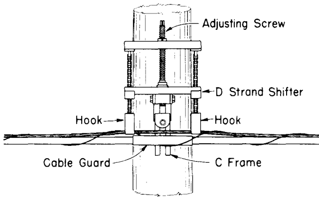
Fig. 14—D Strand Shifter Installed on C Cable Block Frame
