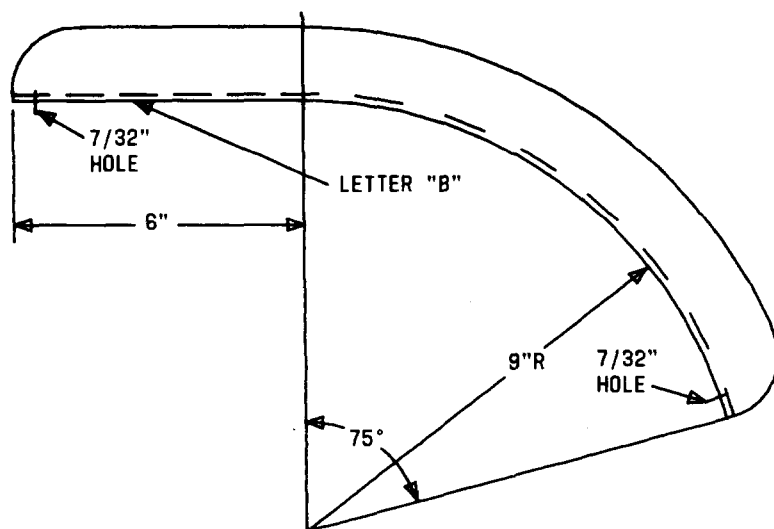
Fig. 1—B Cable Bending Shoe
