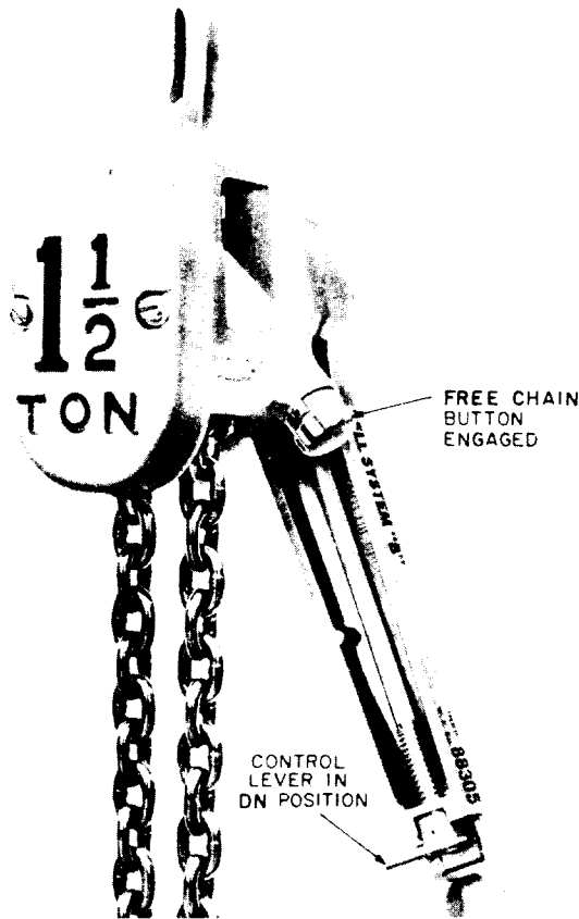
Fig. 5 — Control Lever and FREE CHAIN Button Positioned for Lowering Load
