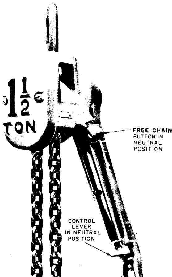
Fig. 3 — Control Lever and FREE CHAIN Button Positioned for Free Chaining
