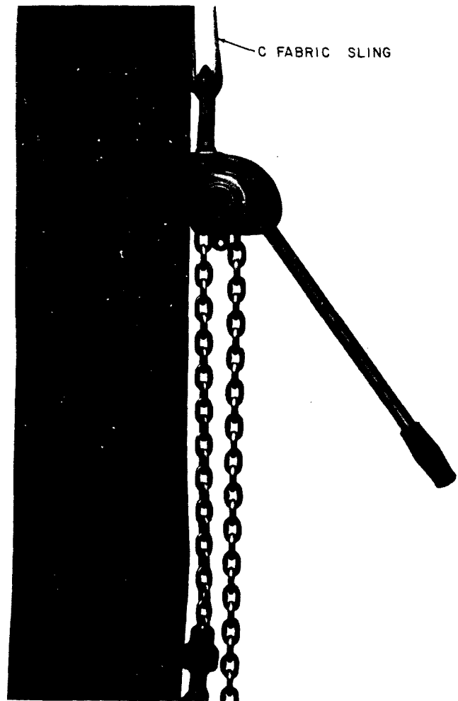
Fig. 4—Vertical Position
