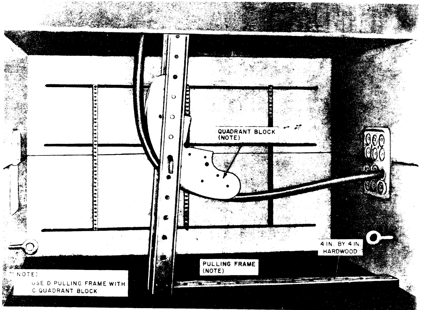
Fig. 2—Pulling Arrangement Using Pulling Frame and Quadrant Block
