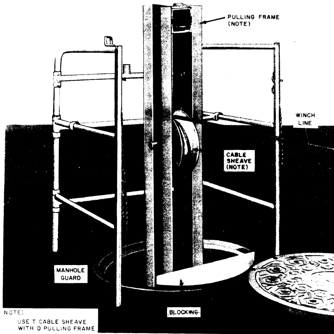
Fig. 3—View Above Manhole Showing Pulling Frame and Cable Sheave
