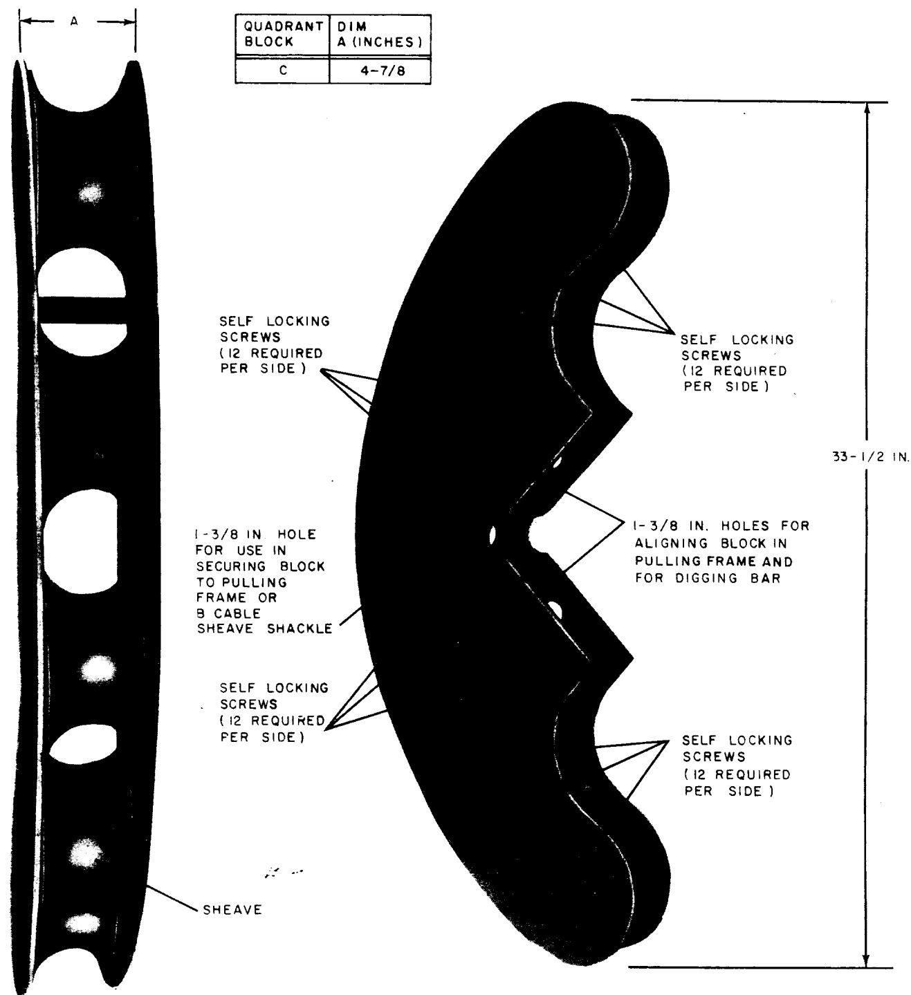
Fig. 1—C Quadrant Block
