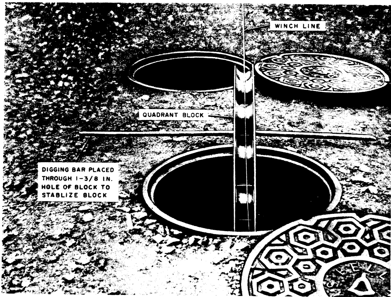
Fig. 4—Quadrant Block Positioned on Edge of Manhole
