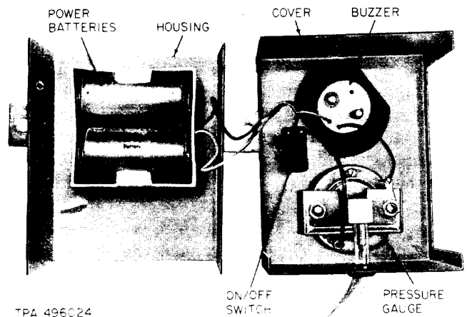
Fig. 10—Cable Reel Pressure Alarm (With Cover Removed)
