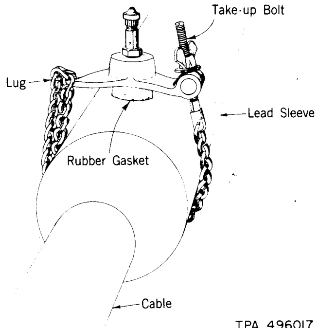
Fig. 3—Pressure Testing Clamp
