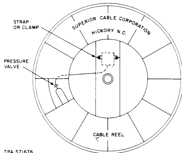
Fig. 11—Cable Reel Pressure Alarm Attached to Reel
