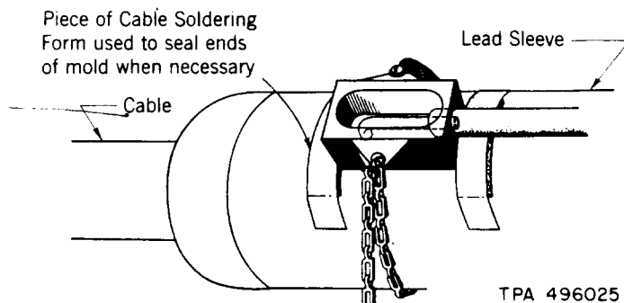
Fig. 12—Lead Pipe Soldering Mold
