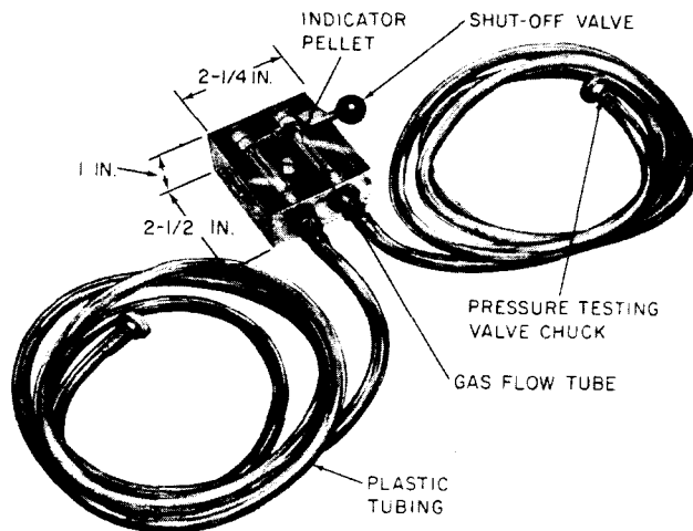
Fig. 5—Airflow Indicator
