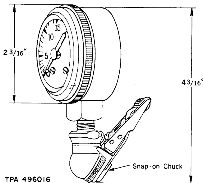
Fig. 1—B Pressure Gauge
