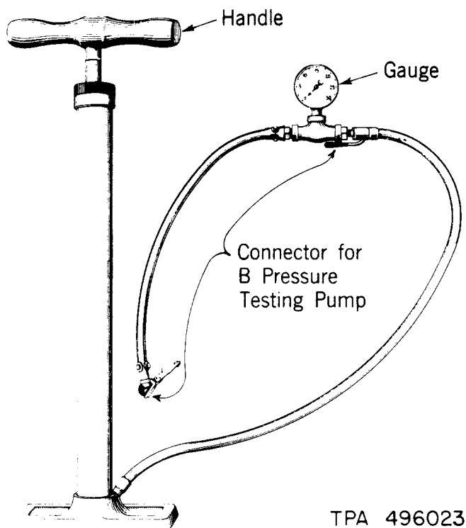
Fig. 8—B Pressure Testing Pump
