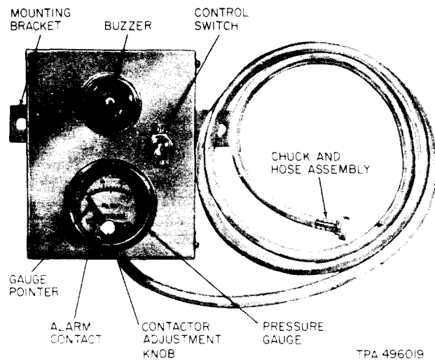
Fig. 9—Cable Reel Pressure Alarm
