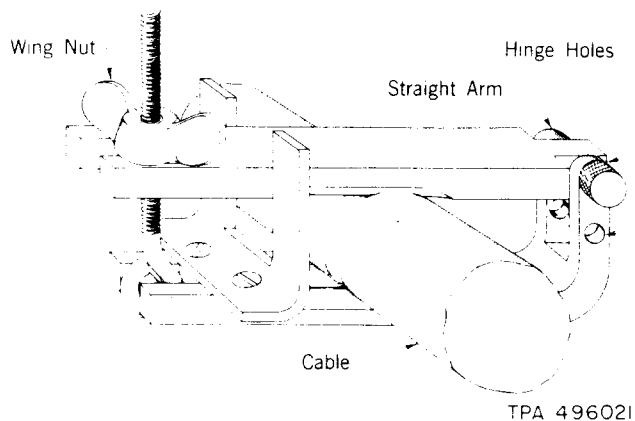
Fig. 7—B Cable Sheath Constrictor
