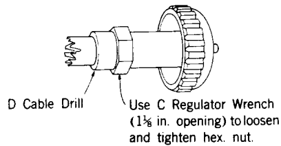
Fig. 5 — Replacing Bit for D Cable Drill
