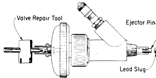
Fig. 3 — Removing Lead Slug from B and C Cable Drills
