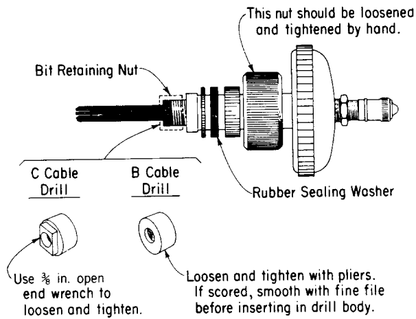
Fig. 4 — Replacing Bit for B and C Cable Drills
