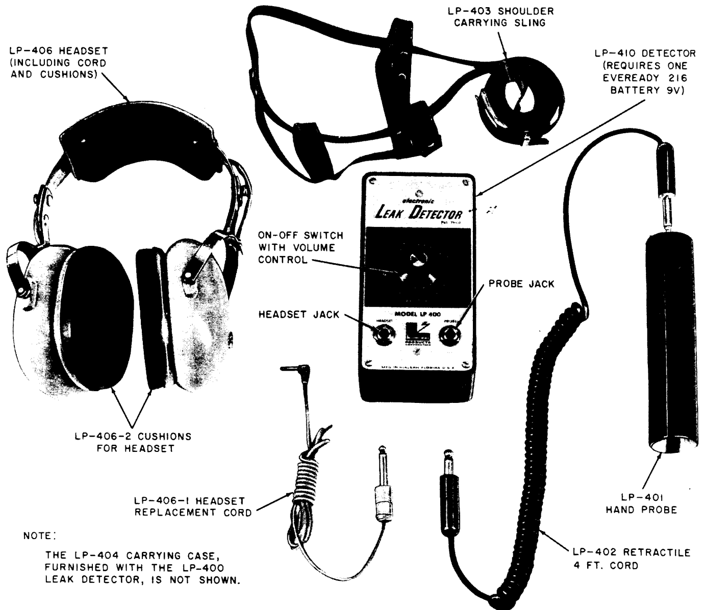
Fig. 9—Lumidor LP-400 Leak Detector
