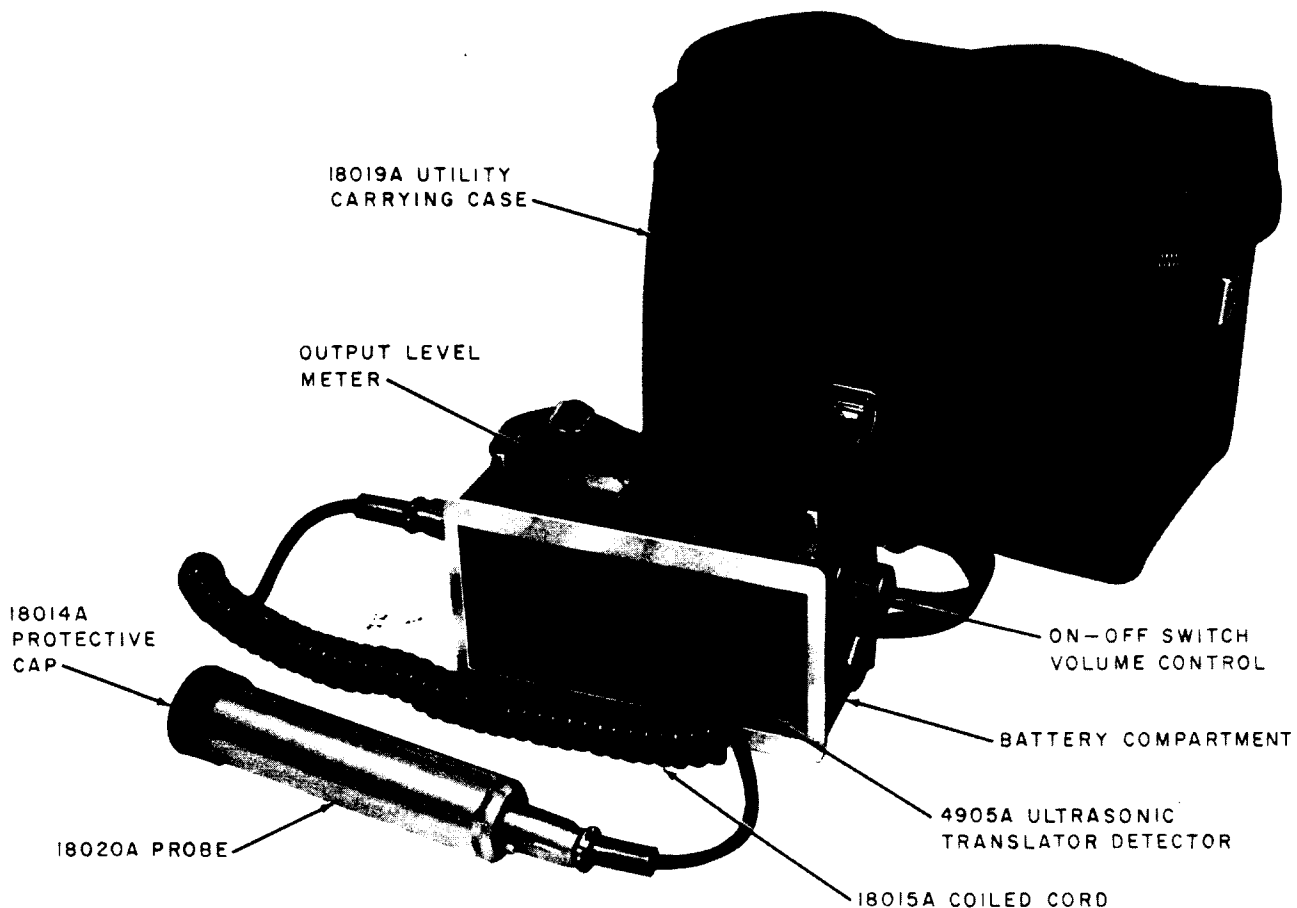
Fig. 2—Hewlett-Packard Delcon Division 4905A Ultrasonic Translator Detector
