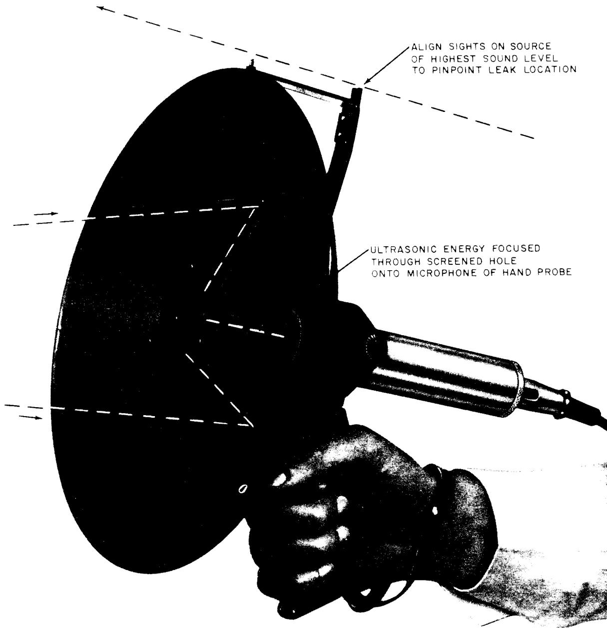
Fig. 15—B Ultrasonic Reflector—Principle of Operation
