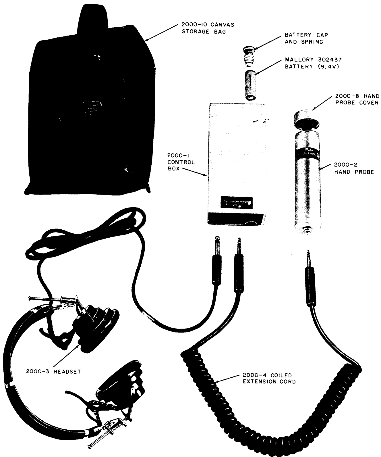
Fig. 12—Malor Group A ULT 2000 Ultrasonic Leak Locator
