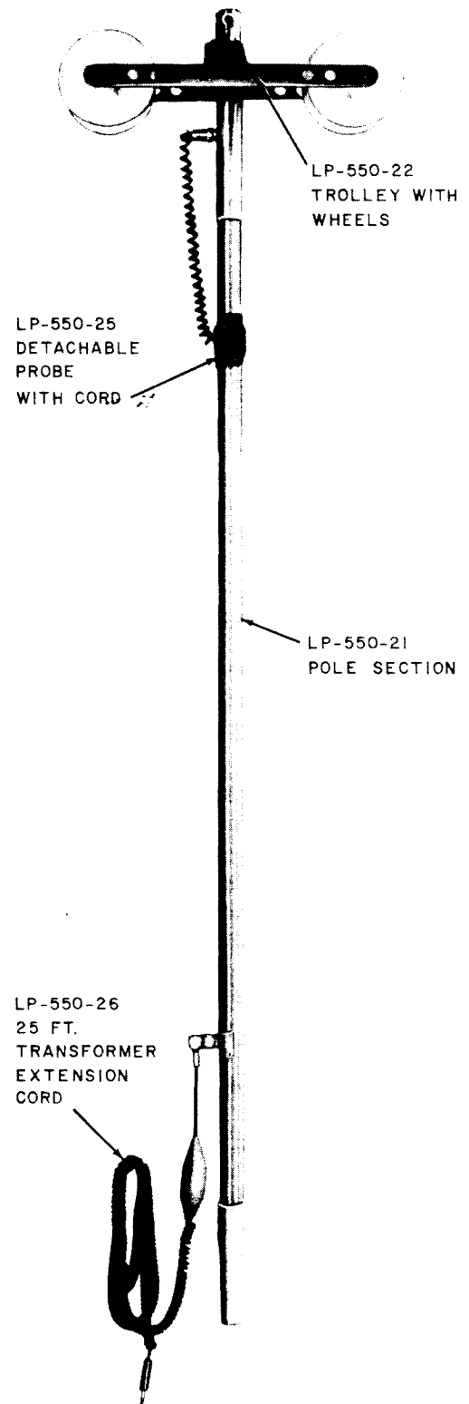
Fig. 7—Lumidor LP-560 Overhead Trolley
