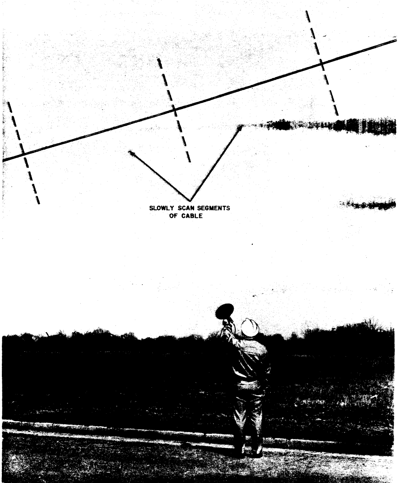
Fig. 16—Scanning Cable Segments with B Ultrasonic Reflector
