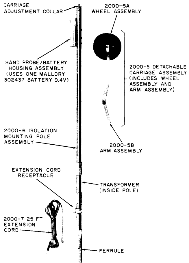
Fig. 13—Malor Group B ULT 2000 Aerial Assembly
