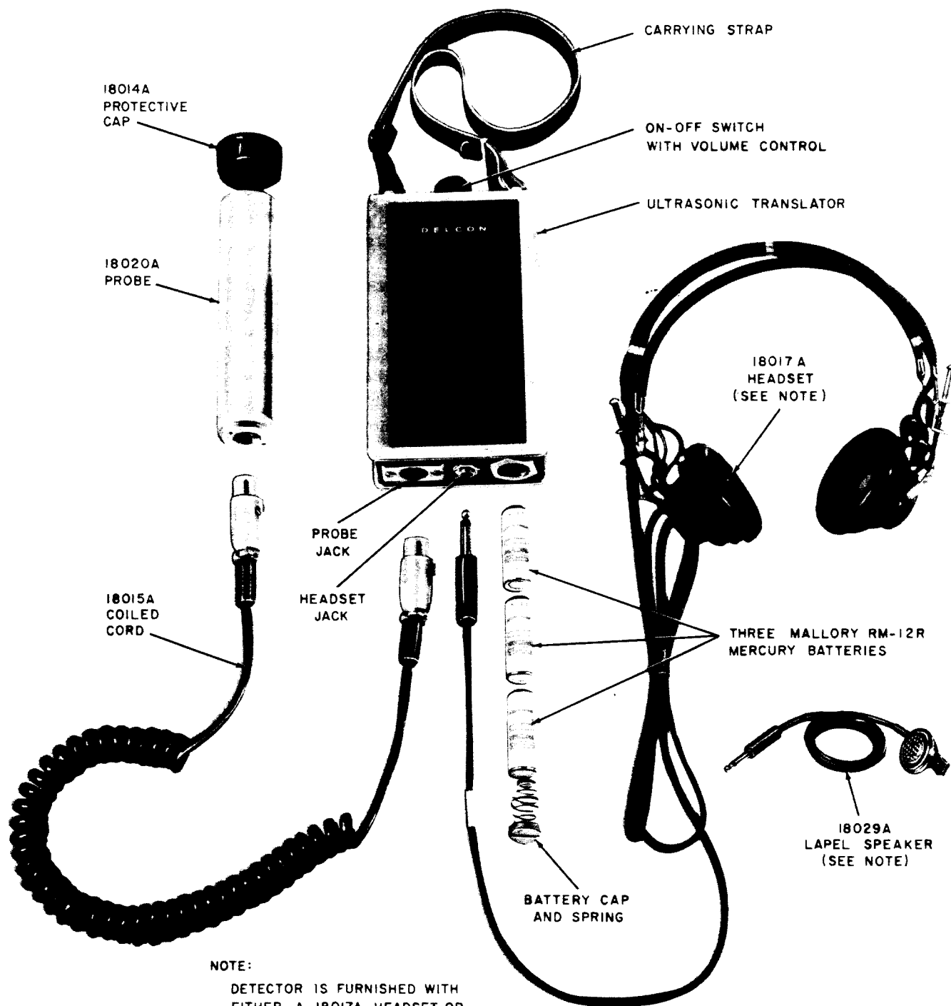
Fig. 1—Hewlett-Packard Delcon Division 4916A Ultrasonic Translator Detector
