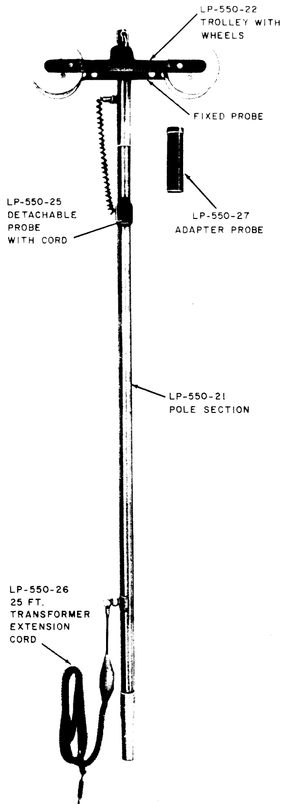
Fig. 6—Lumidor LP-550 Overhead Trolley and Pole Probe
