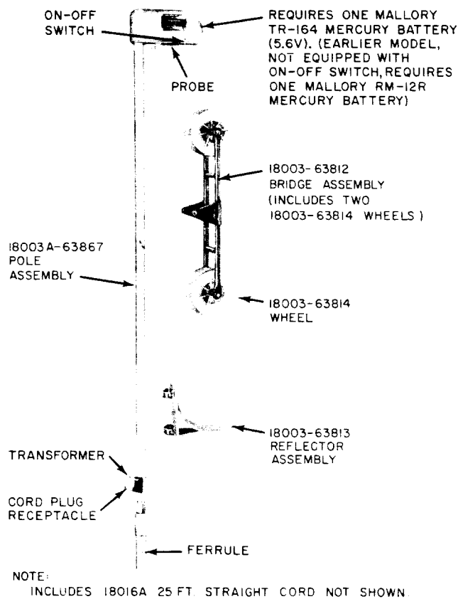
Fig. 3—Hewlett-Packard Delcon Division 18003A Mobile Reflector
