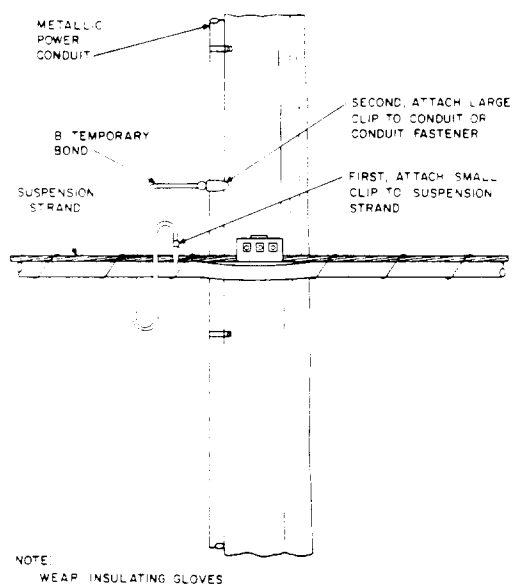
Fig. 15--Temporary Bond Attachment to Metallic Power Conduit
