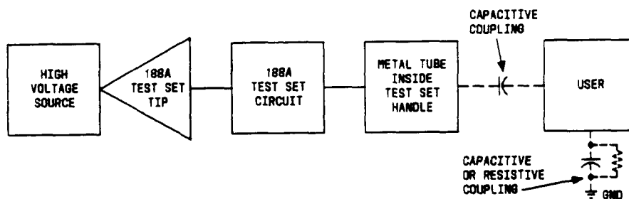
Fig. 6--Current Path
