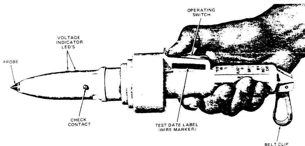
Fig. 7--Proper Grip of 188A Test Set
