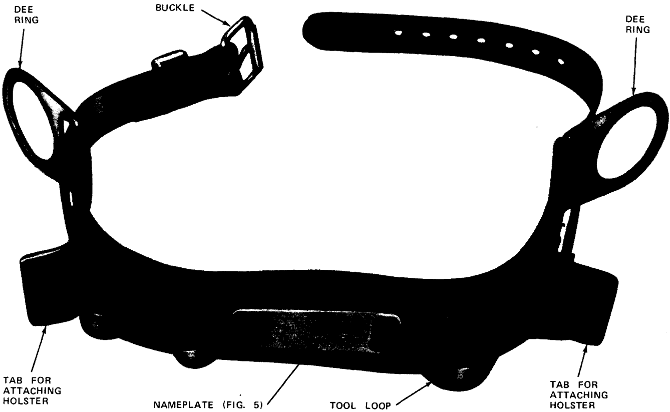
Fig. 2—F Body Belt
