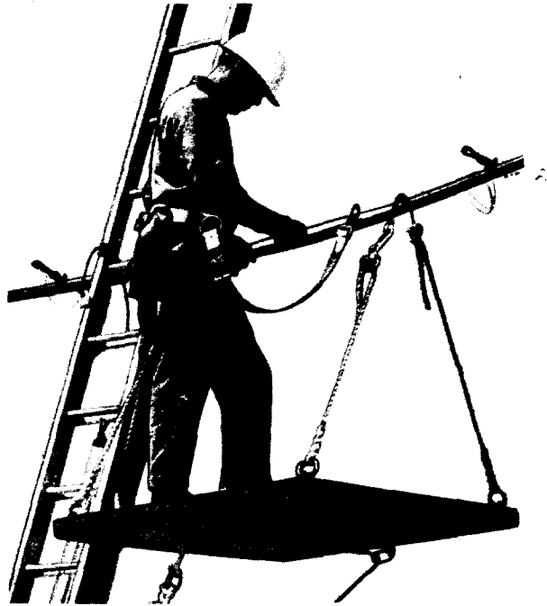
Fig. 8—Method of Using Safety Strap When Using Other Than a D, E, or F Belt
