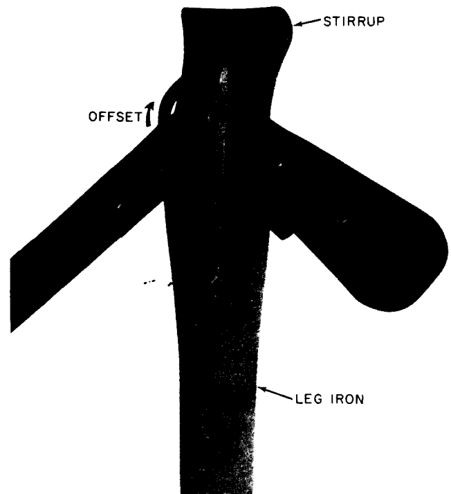
Fig. 2—Stirrup Offset "Right"
