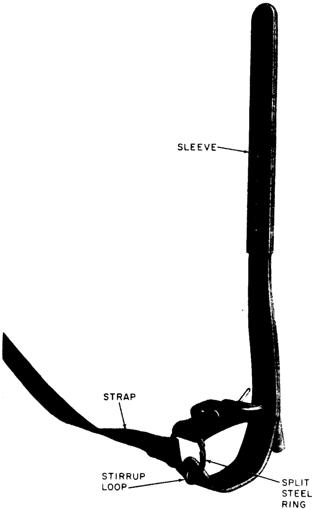
Fig. 6—Foot Straps Attached to Climbers
