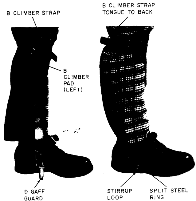
Fig. 10—Climber Strapped to Leg
