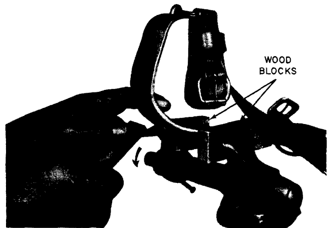
Fig. 21—Using Vise for Honing Gaff
