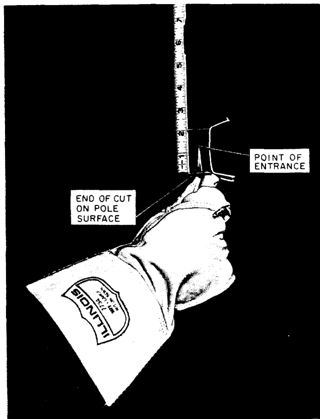
Fig. 16—Measuring Gaff Cut
