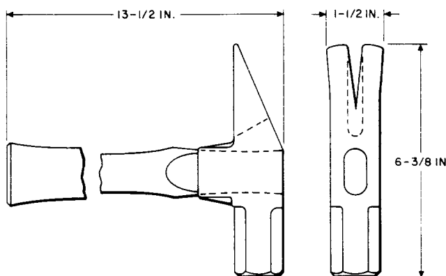
Fig. 3—Two Pound Claw Hammer
