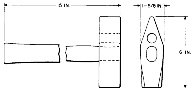
Fig. 11—Three Pound Driving Hammer
