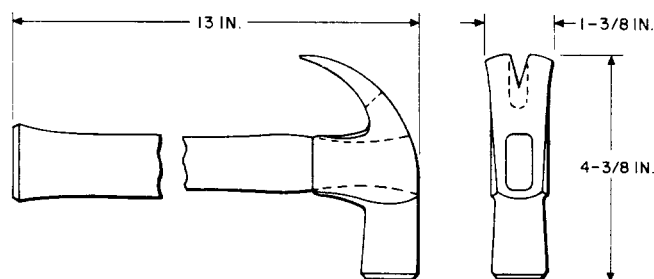
Fig. 1—One Pound Claw Hammer
