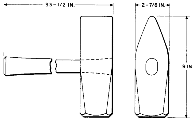
Fig. 10—Sixteen Pound Stone Sledge
