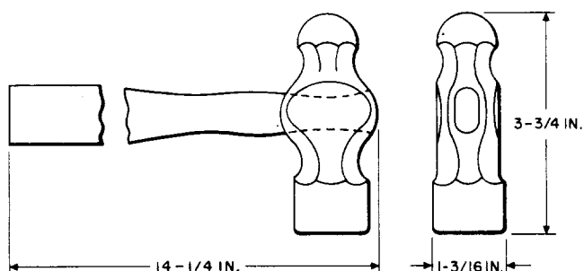
Fig. 4—One Pound Ball Peen Hammer
