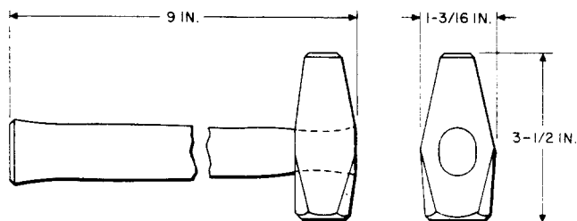
Fig. 5—One and One-Quarter Pound Drilling Hammer
