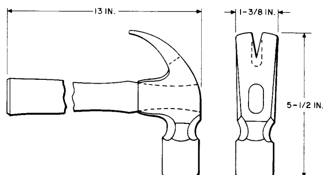
Fig. 2—One and One-Half Pound Claw Hammer
