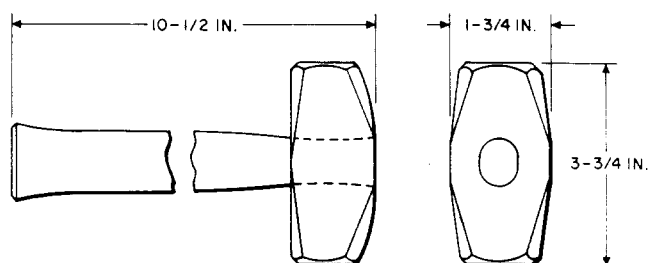
Fig. 6—Two Pound Drilling Hammer
