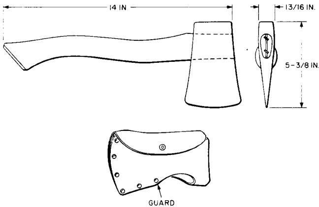
Fig. 13—One and One-Quarter Pound Hatchet and Guard
