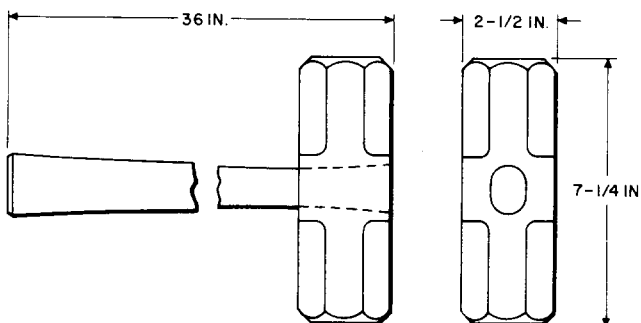
Fig. 9—Ten Pound Blacksmith Sledge
