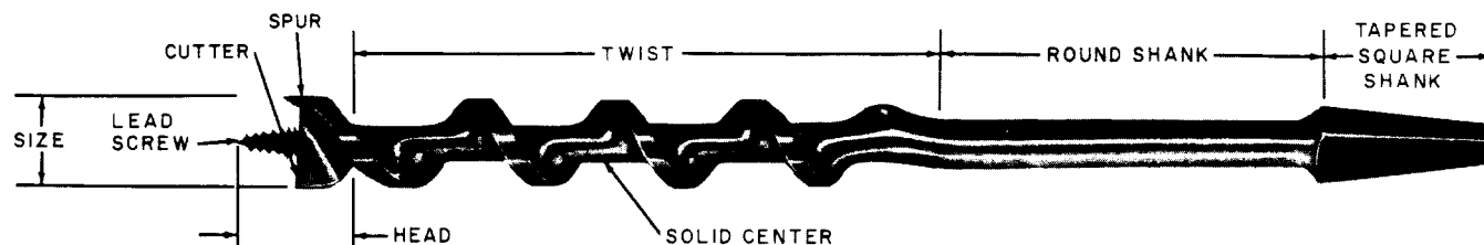
Fig. 1 — Auger Bit
