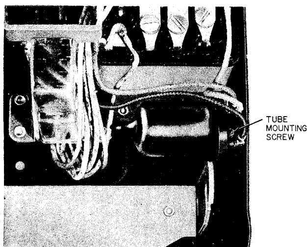
Fig. 21 — 501-Type Telephone Set, Tube Assembly
