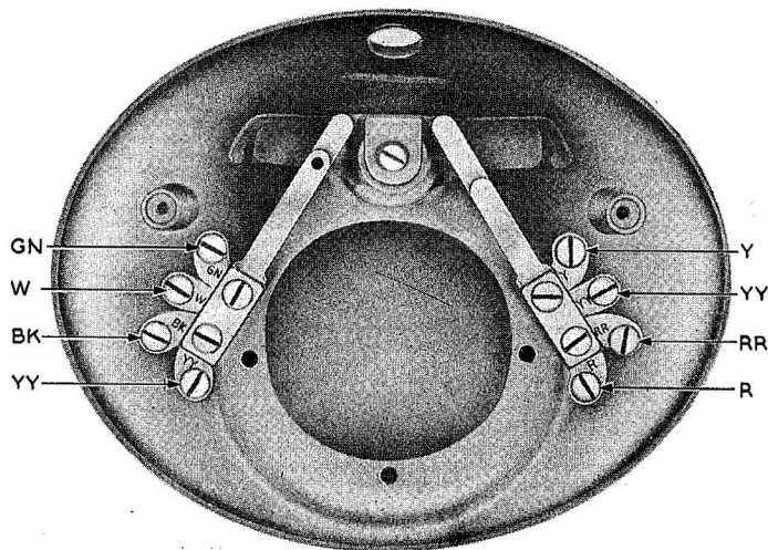
FIG. 5—D6-TYPE HANDSET MOUNTING
