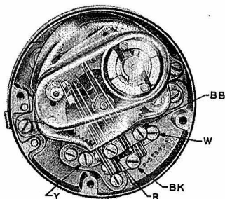
FIG. 3—6A-TYPE DIAL
