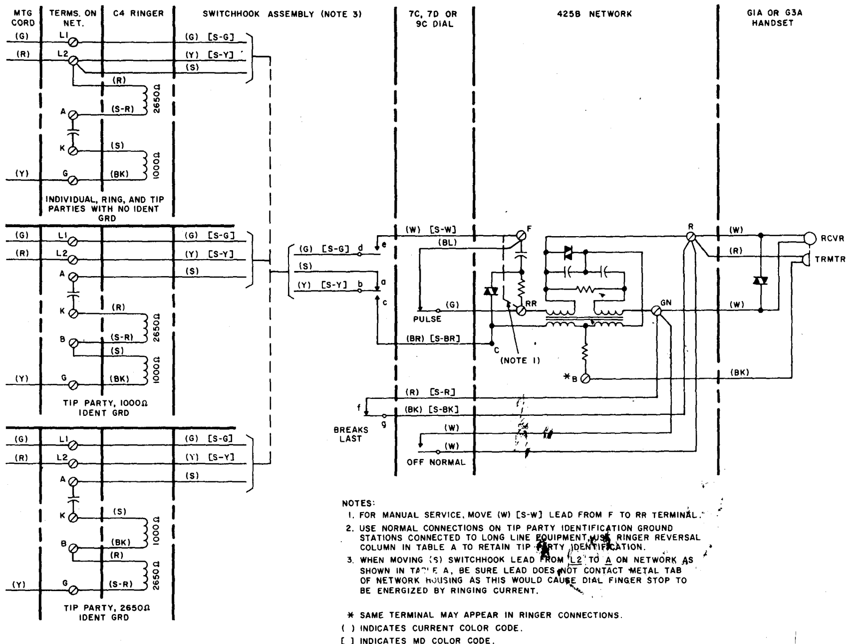
Fig. 1 — 500C and D Telephone Sets, Connections TCI Library: www.telephonecollectors.info
