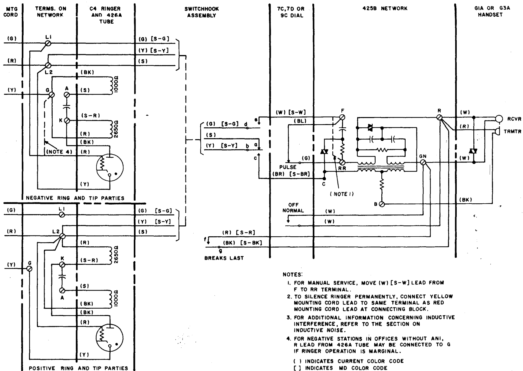
Fig. 2 — 501C and D Telephone Sets, Connections
