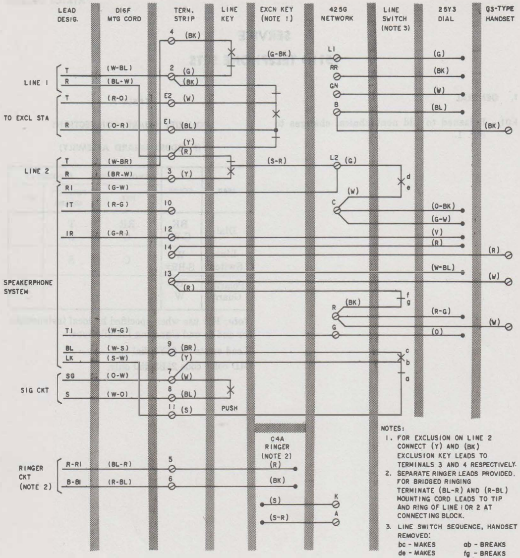
Fig. 1—1511D (MD) Telephone Set Connections, Equipped With 25Y3 (MD) Dial
