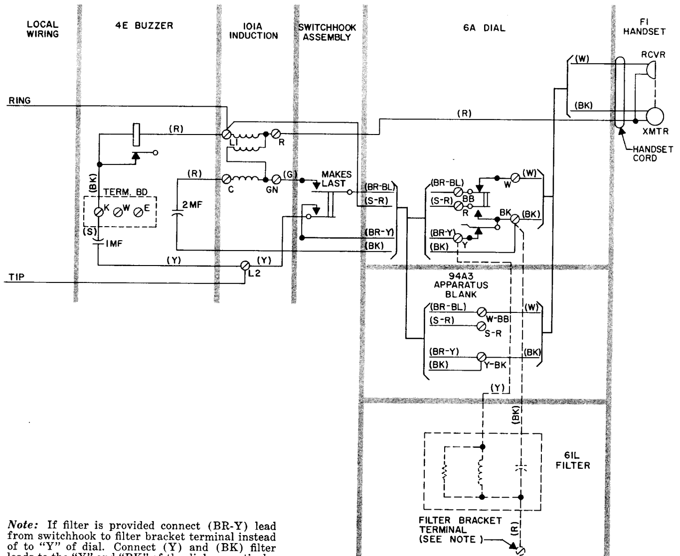
Fig. 5 — 322-Type Telephone Set, Connections
