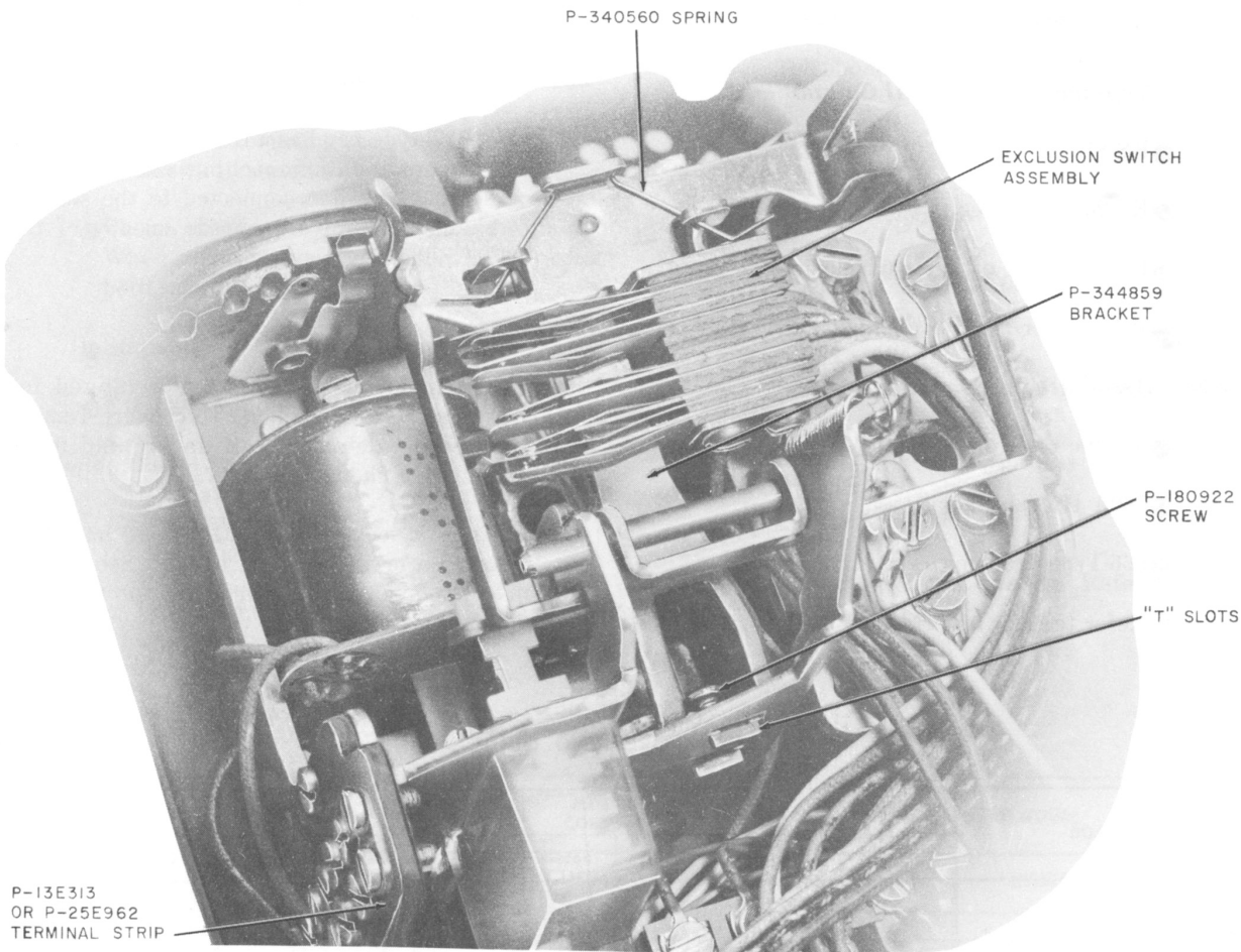
Fig. 3—D-179935 Exclusion Kit, Installed
