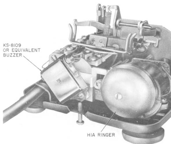
Fig. 8—Location of KS-8109L2 Buzzer
