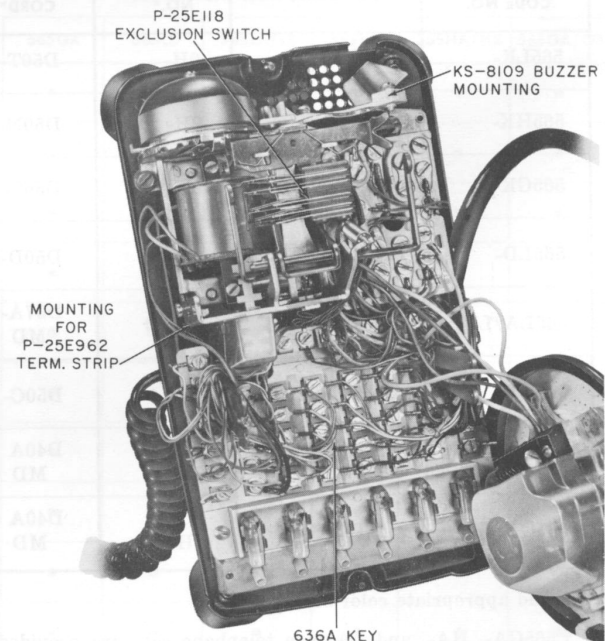
Fig. 2—565HK Telephone Set, Interior
