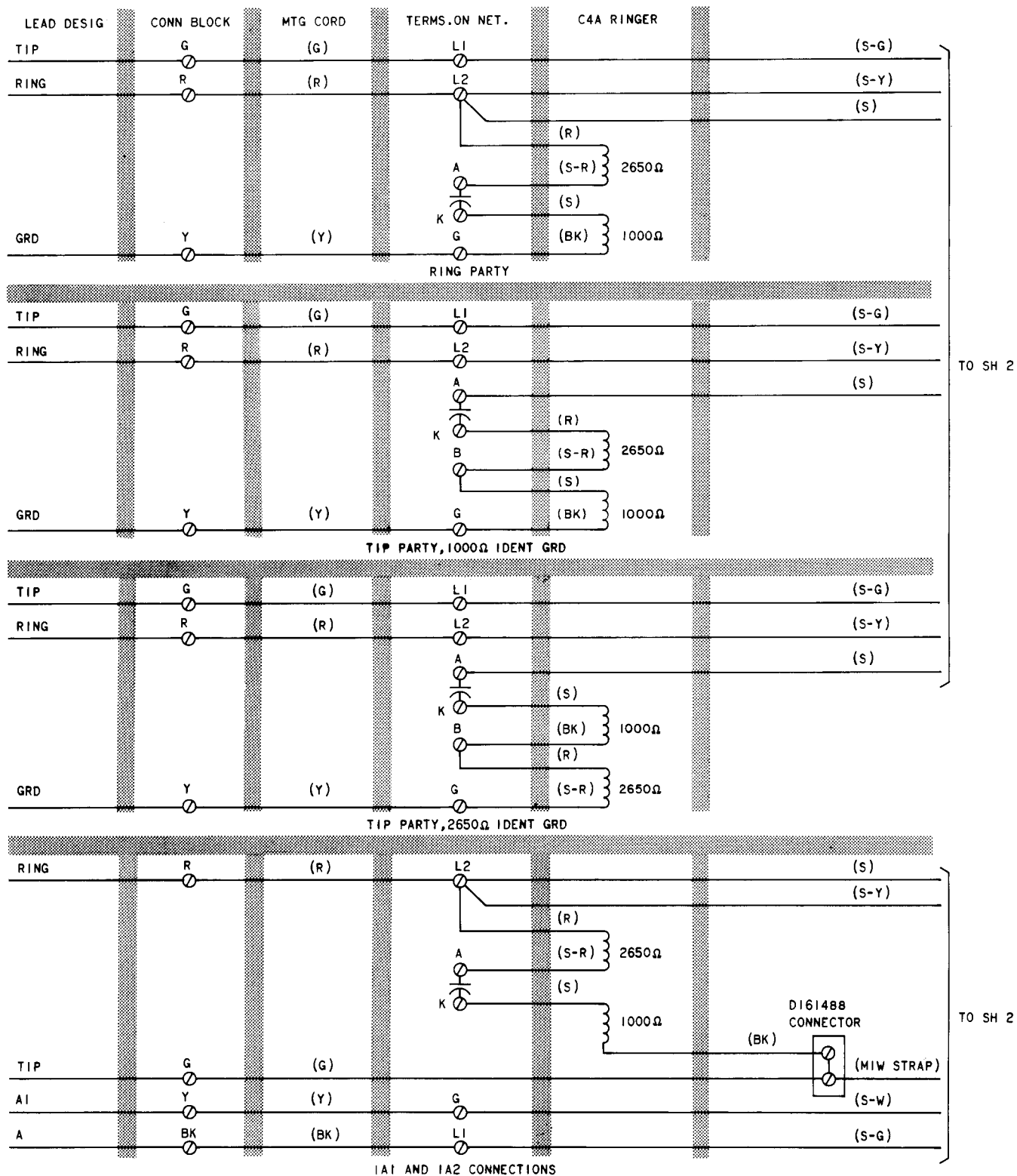
Fig. 15—535A and B Telephone Sets, Connections (Sheet 1 of 2)
