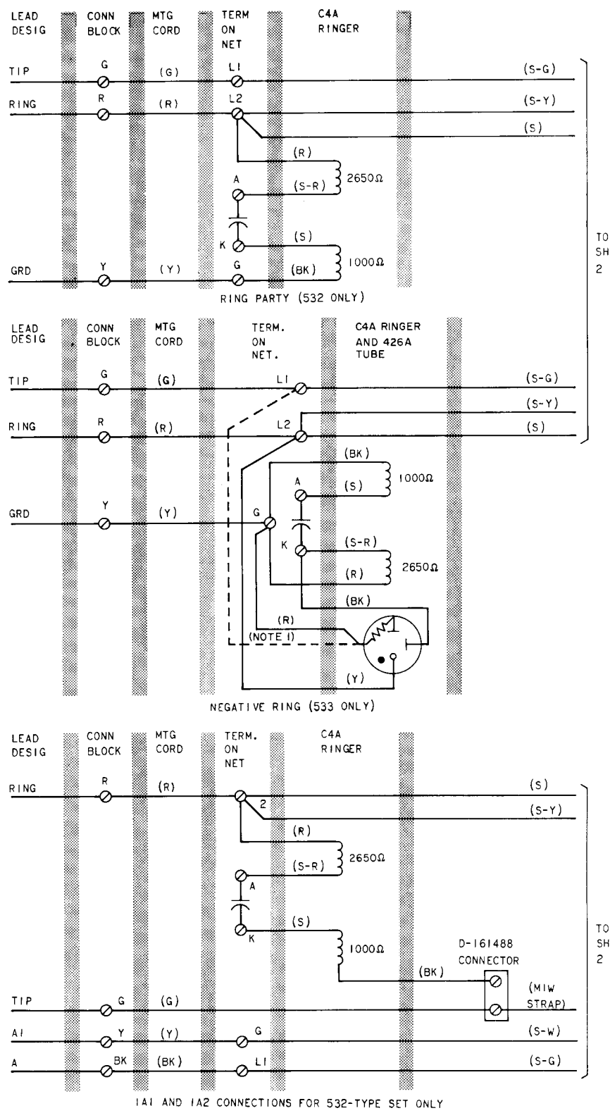
Fig. 14—532- and 533-Type Sets, Connections (Sheet 1 of 2)
