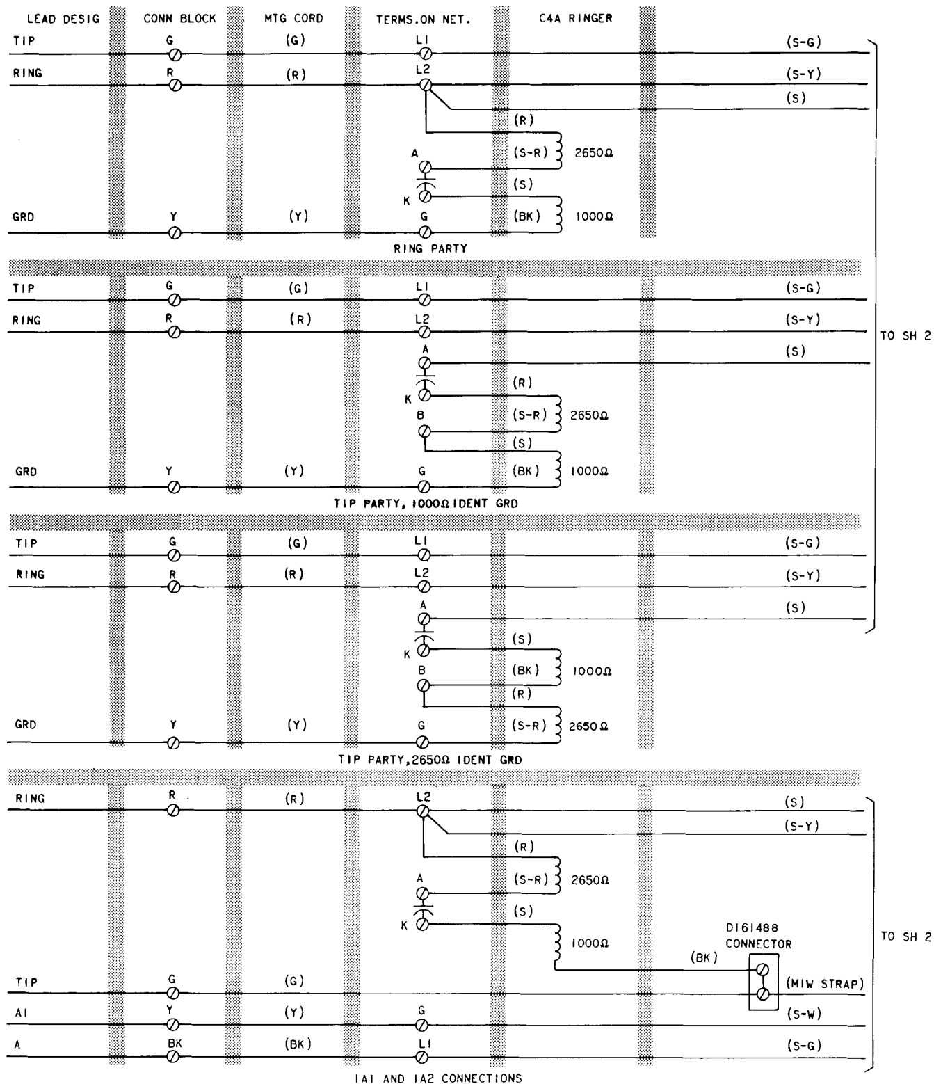
Fig. 16—536A and B Telephone Sets, Connections (Sheet 1 of 2)
