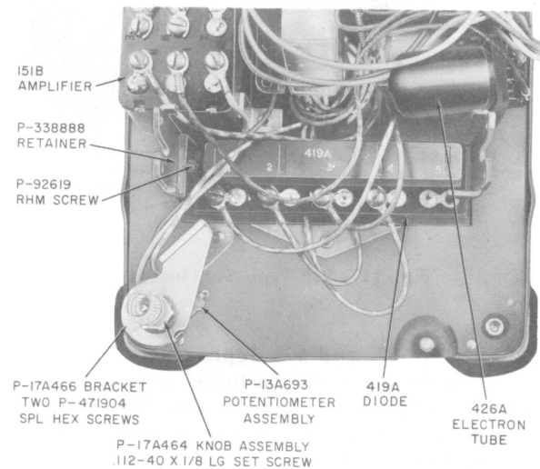
Fig. 9—533-Type Set, Exterior
