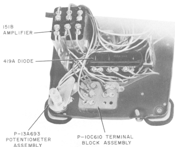
Fig. 11—535-Type Set, Interior
