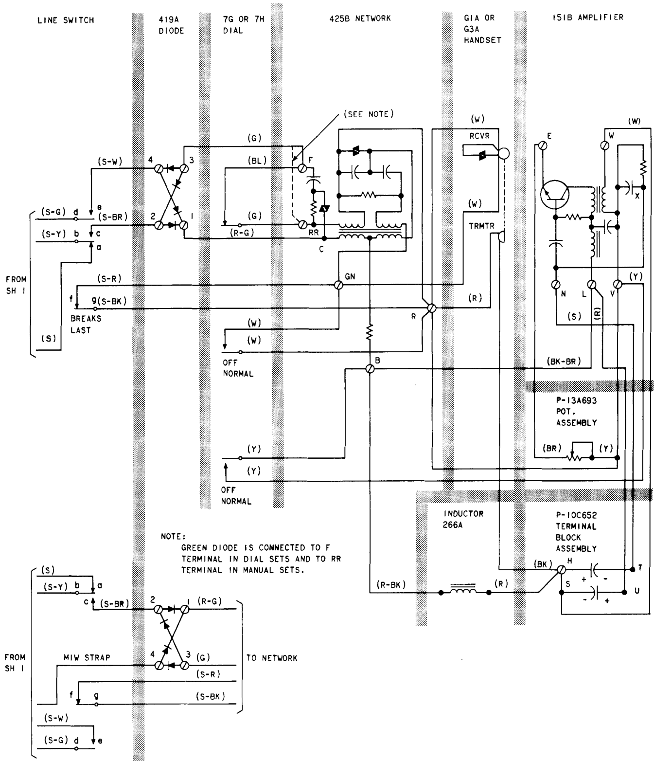
Fig. 16—536A and B Telephone Sets, Connections (Sheet 2 of 2)
