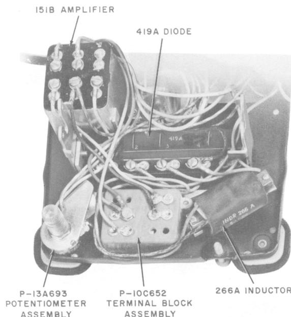
Fig. 12—536-Type Set, Interior
