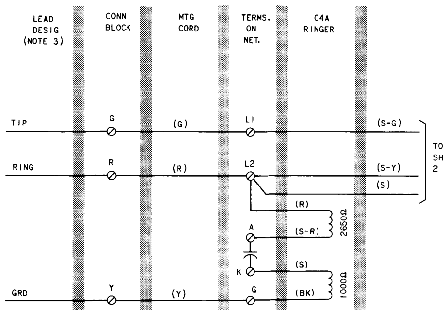
RING PARTY 507- AND 557- TYPE TELEPHONE SETS (NOTE 4)
