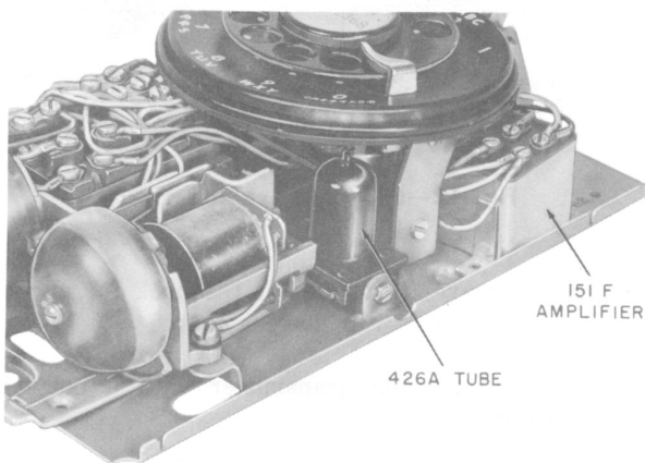
Fig. 6—559-Type Set, Tube Assembly
