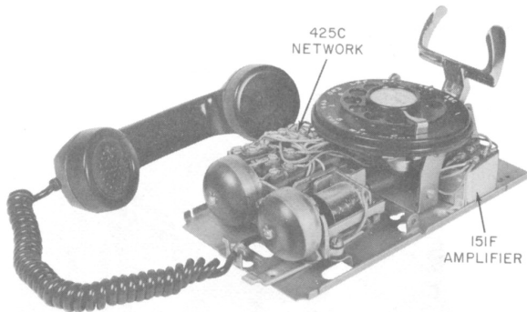
Fig. 5—557-Type Set, Interior
