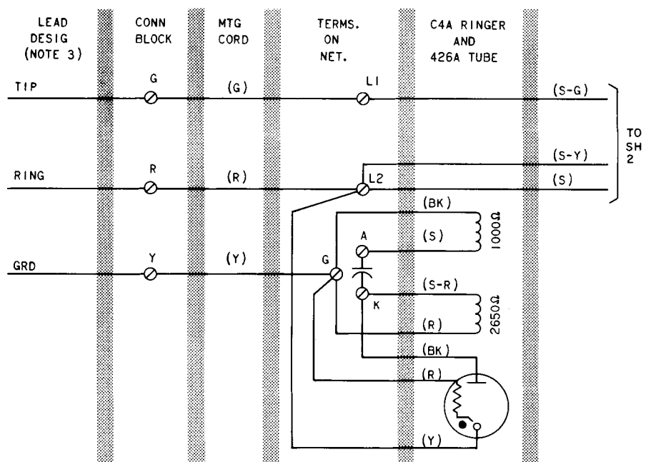
NEGATIVE RING PARTY 509- AND 559- TYPE TELEPHONE SETS (NOTE 5)
