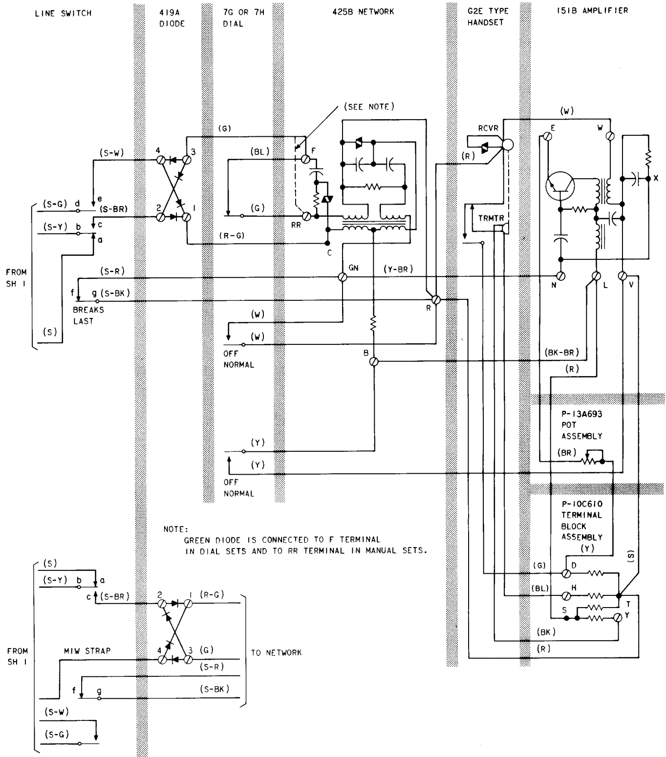
Fig. 15—535A and B Telephone Sets, Connections (Sheet 2 of 2)
