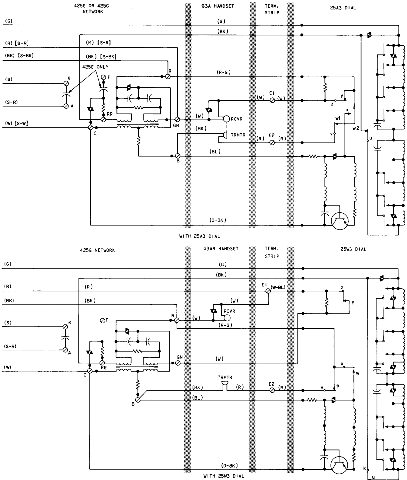
Fig. 2—1500M Telephone Set, Connections (Sheet 2 of 2)
