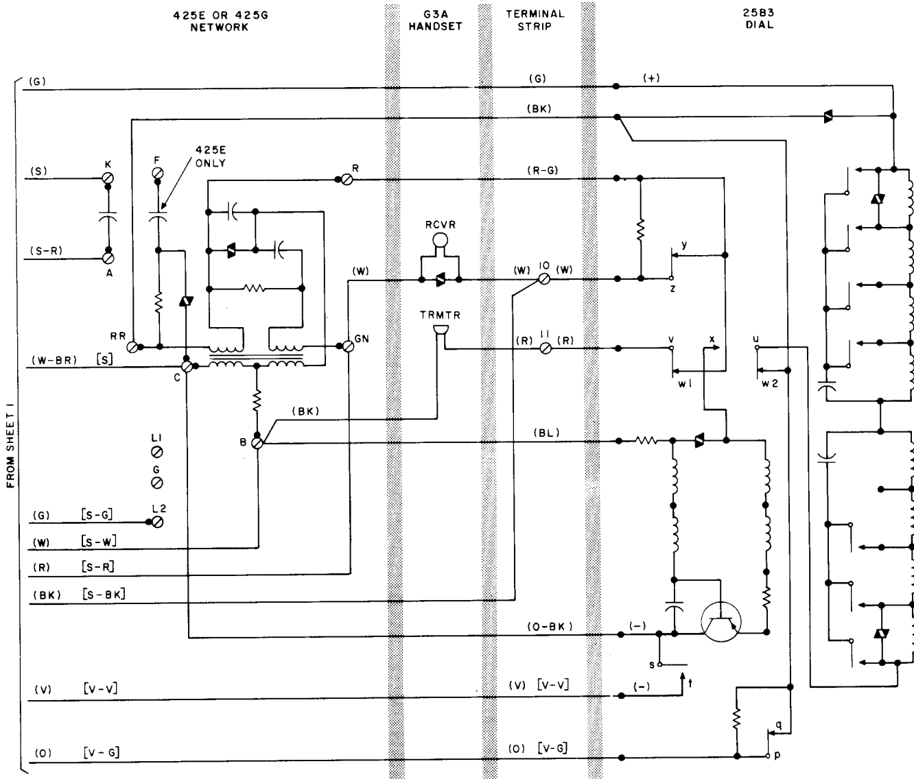
Fig. 3—1500S Telephone Set, Wired for Speakerphone (Sheet 3 of 3)
