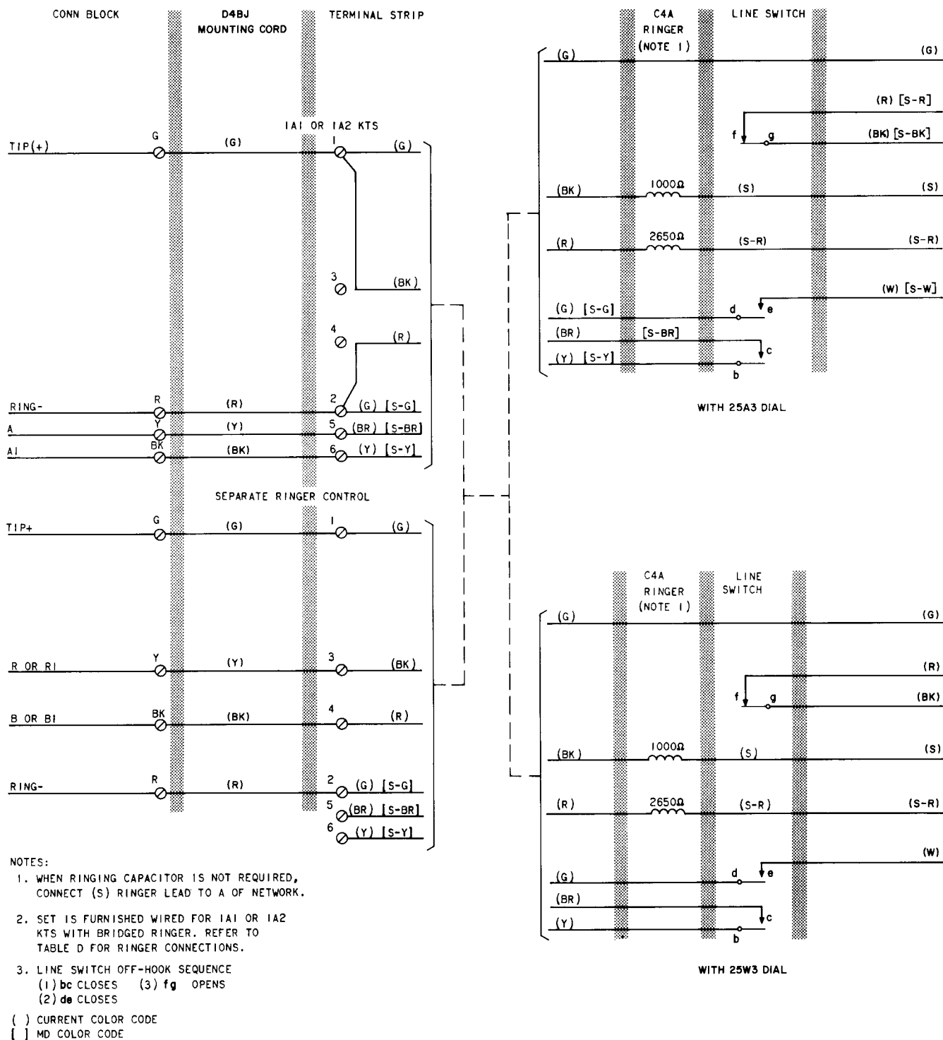
Fig. 2—1500M Telephone Set, Connections (Sheet 1 of 2)
