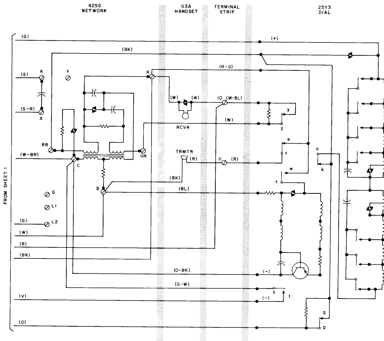
Fig. 3—1500S Telephone Set, Wired for Speakerphone (Sheet 2 of 3)
