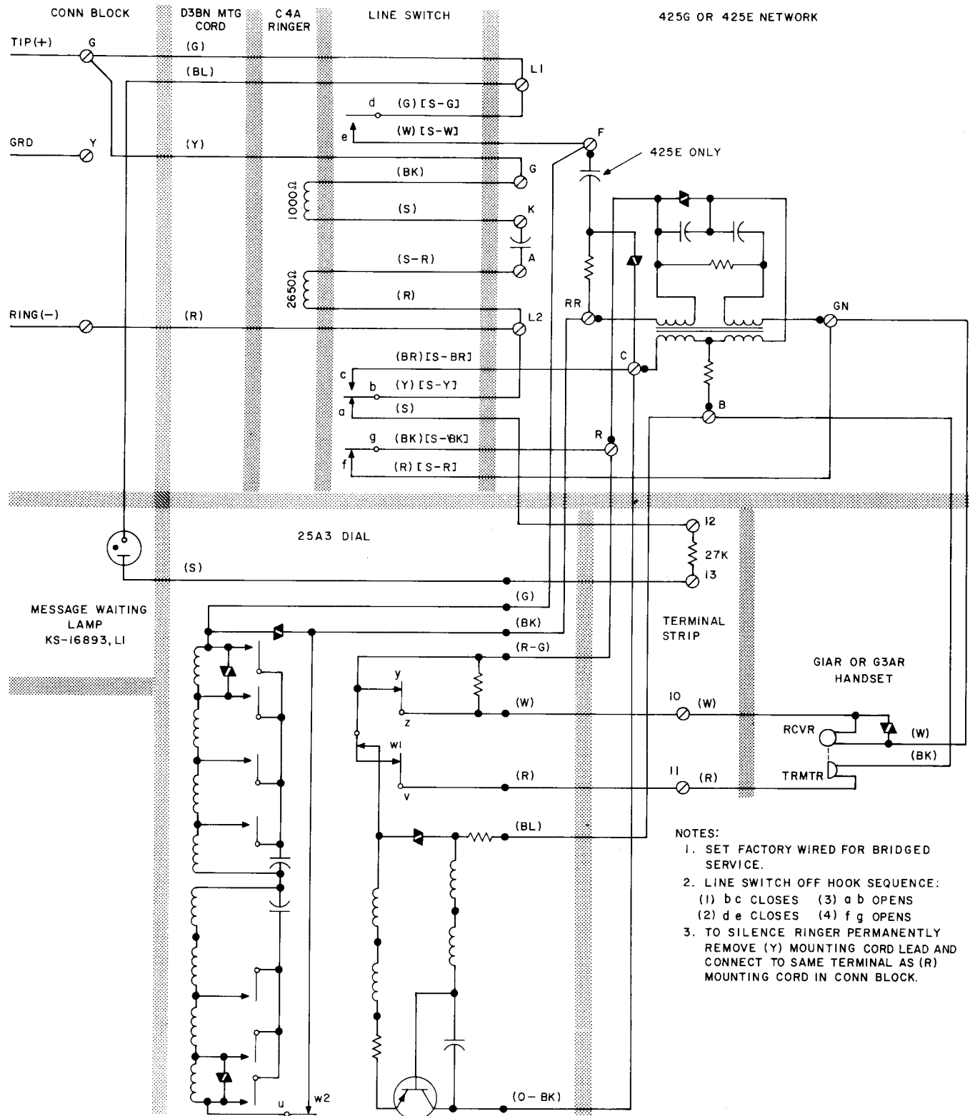
Fig. 4—1500Y Telephone Set, Connections With 25A3 Dial
