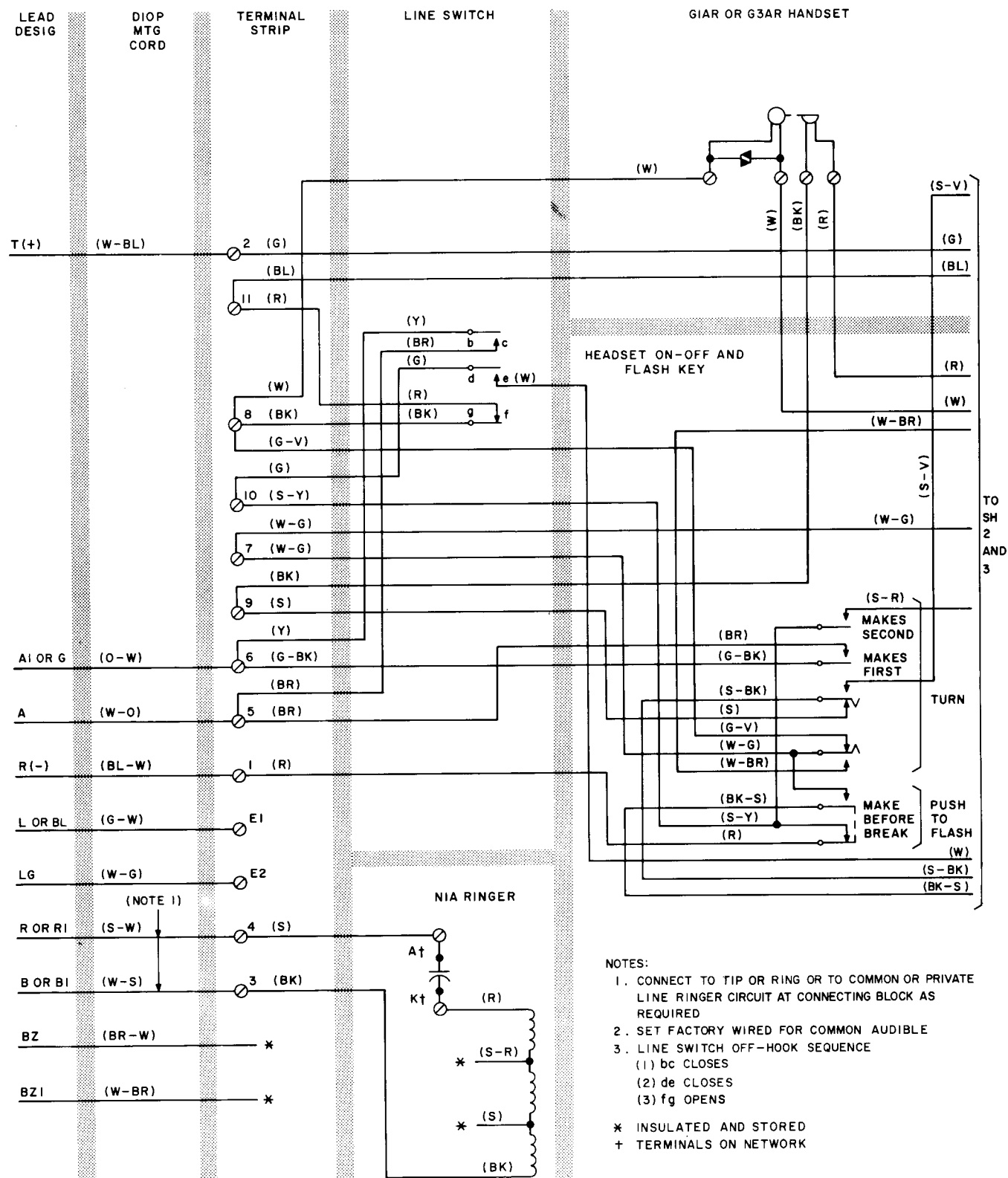
Fig. 6—1514B Telephone Set, Connections (Sheet 1 of 3)
