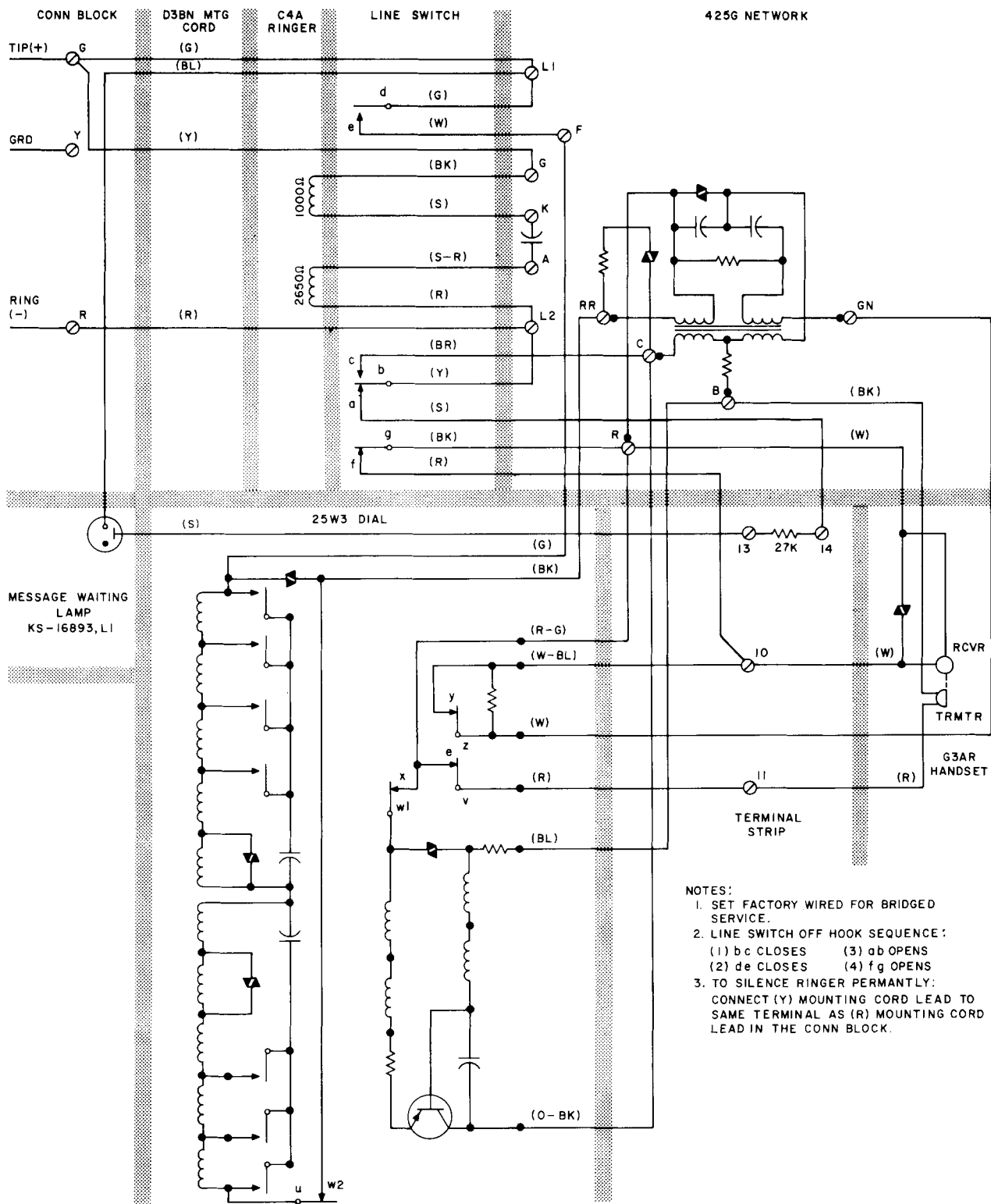
Fig. 5—1500Y Telephone Set, Connections With 25W3 Dial
