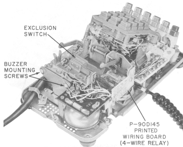
Fig. 5—2568HAA Telephone Set, Interior
