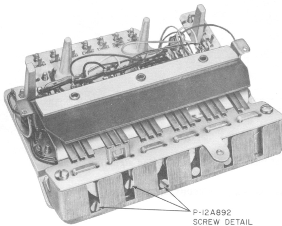
Fig. 7—636A Key, Bottom View
