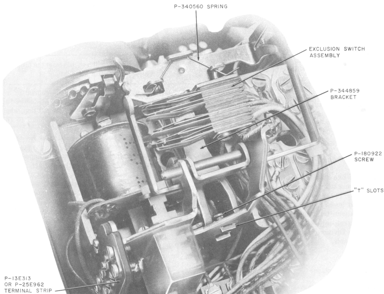
Fig. 2—D-179935 Kit of Parts, Installed
