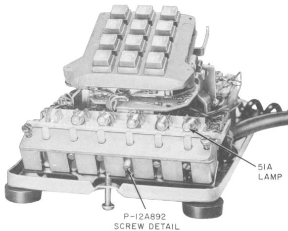
Fig. 4—Location of P-12A892 Screw Detail
