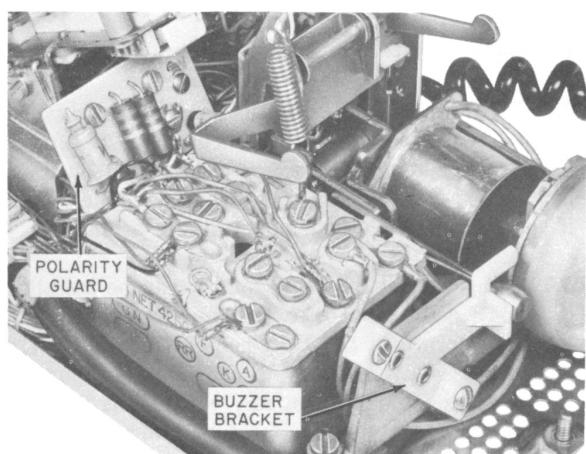
Fig. 3—2565-Type Telephone Set, Interior View
