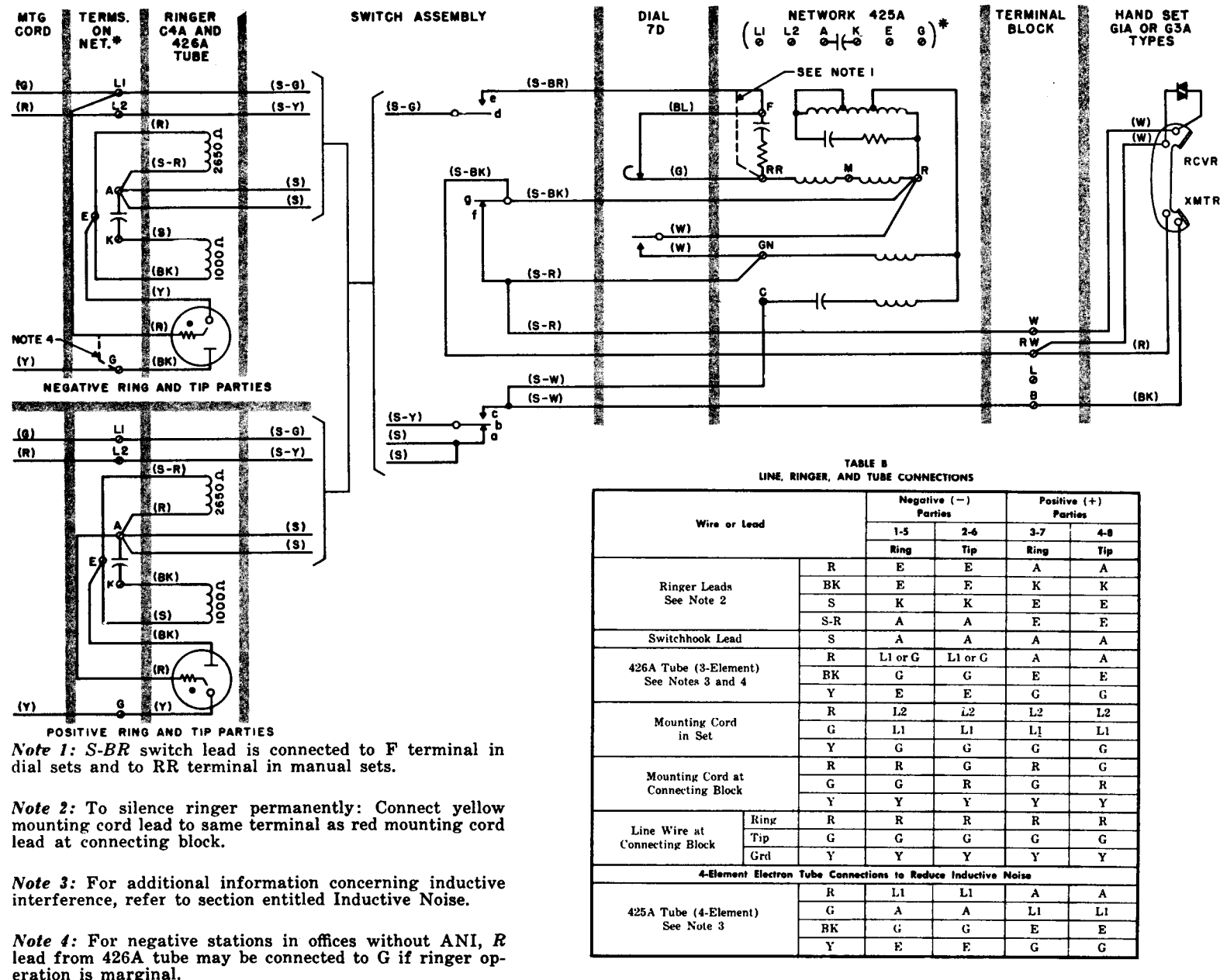
Fig. 2 — 501J, K Telephone Set, Connections
