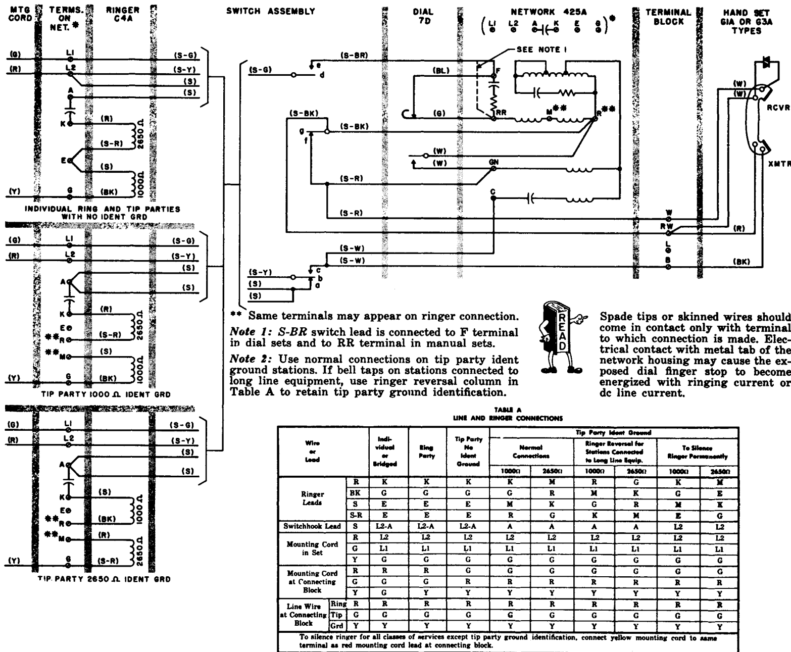
Fig. 1 — 500J, K Telephone Set, Connections
