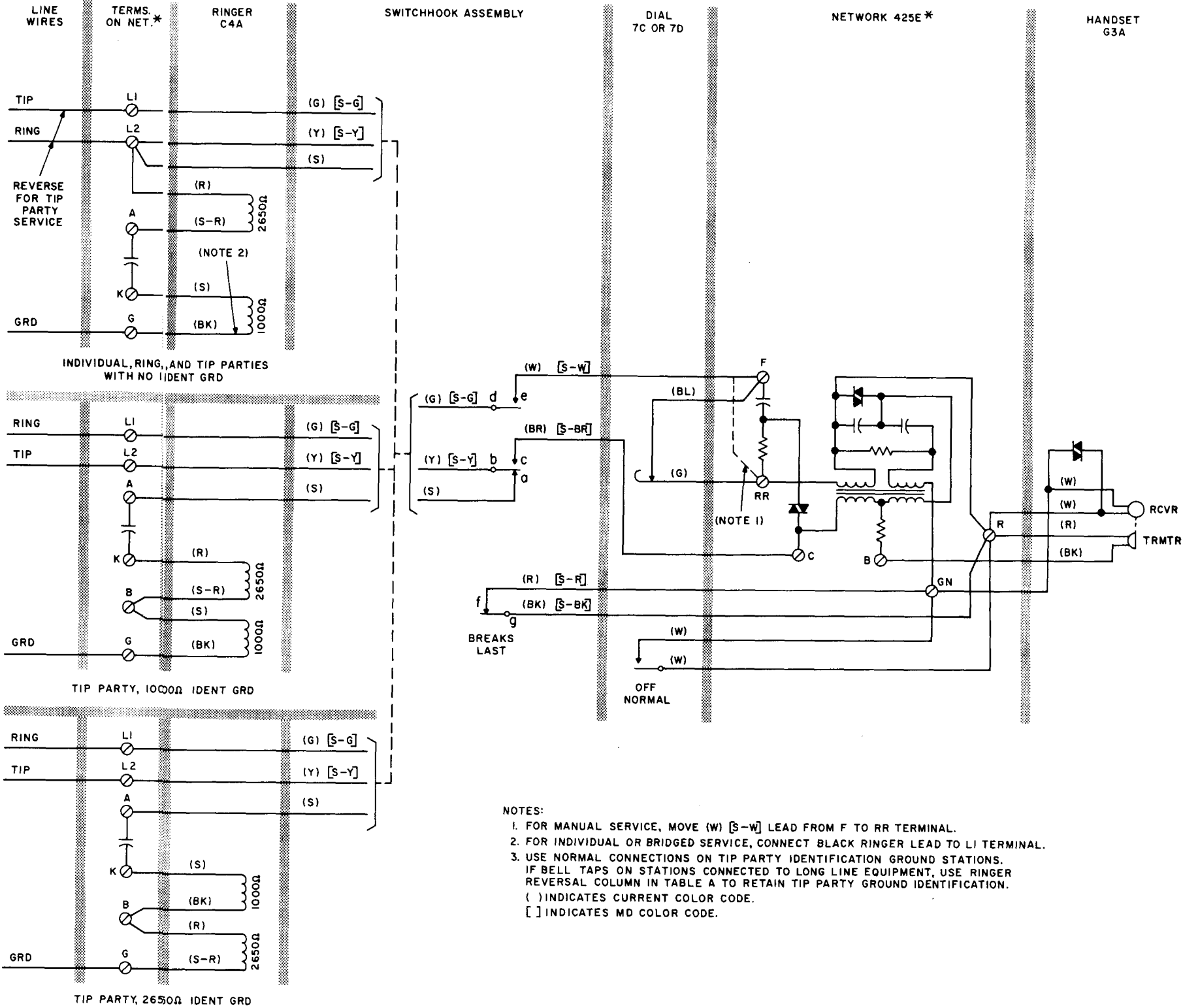
Fig. 1 — 554A and B Telephone Sets, Connections
