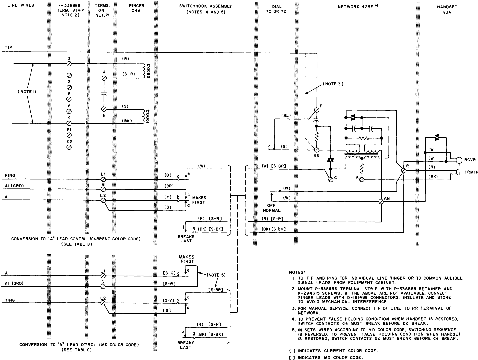
Fig. 2 — 554A and B Telephone Sets Revised for A Lead Control
