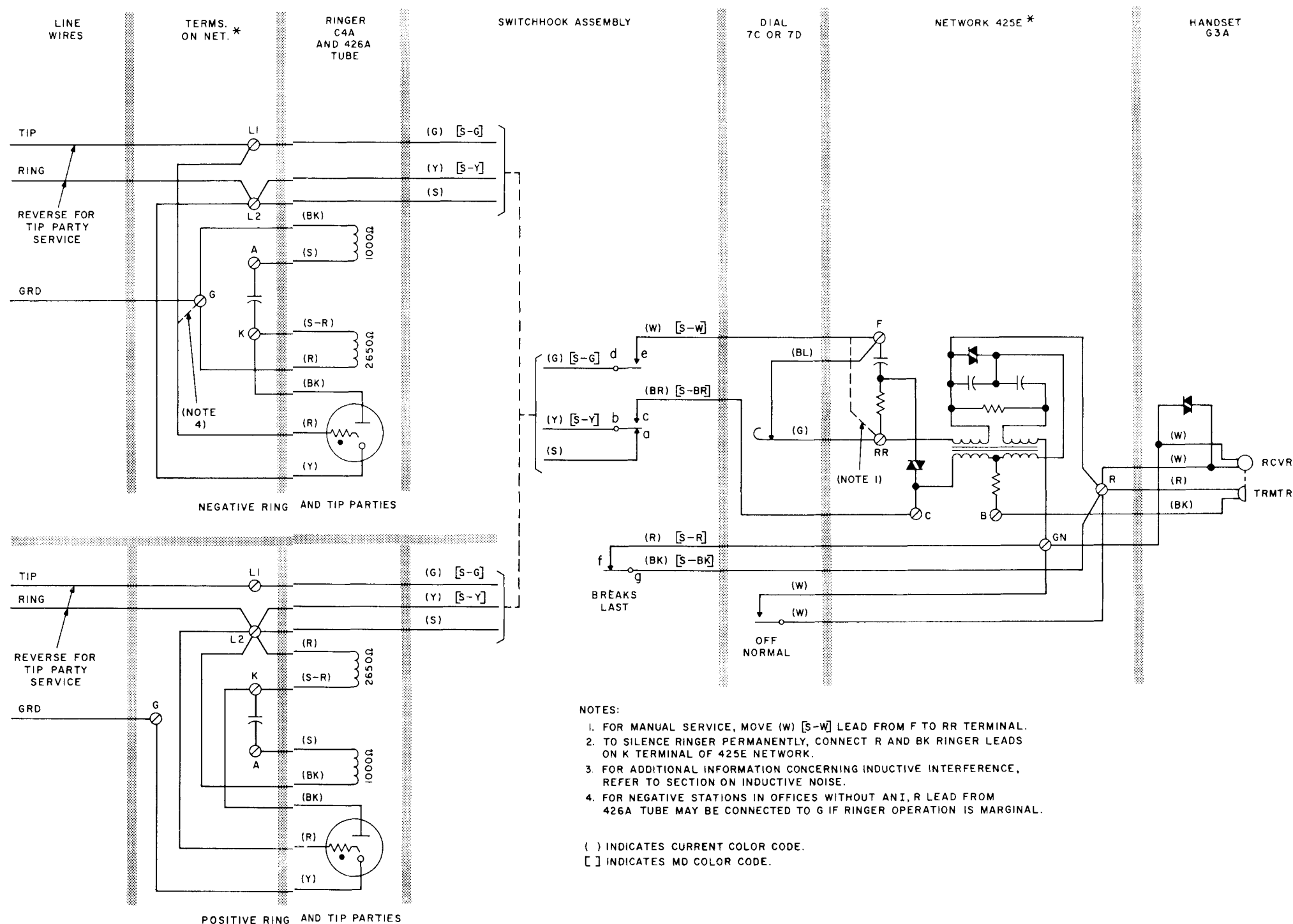
Fig. 3 — 556A and B Telephone Sets, Connections
