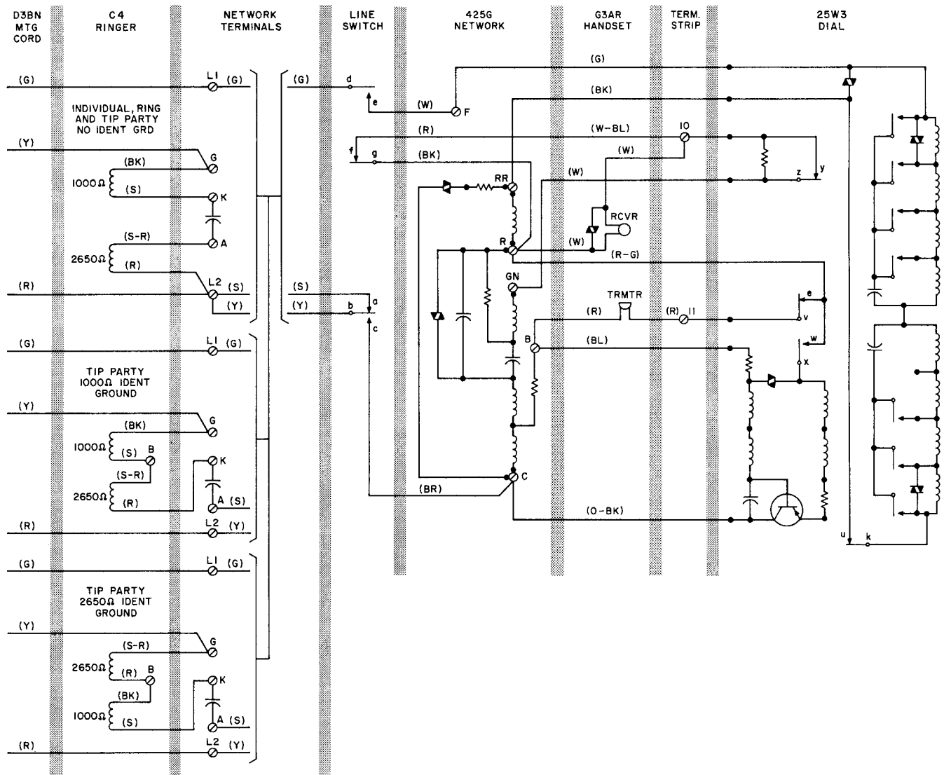
Fig. 2 — 1500D Telephone Set Connections, With 25W3 Dial
