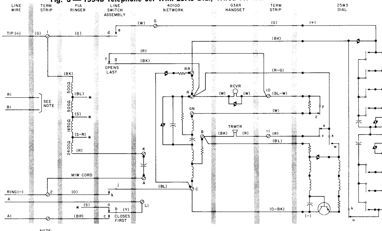
Fig. 3 — 1554B Telephone Set With 25A3 Dial, Wired for 1A1 or 1A2 KTS
