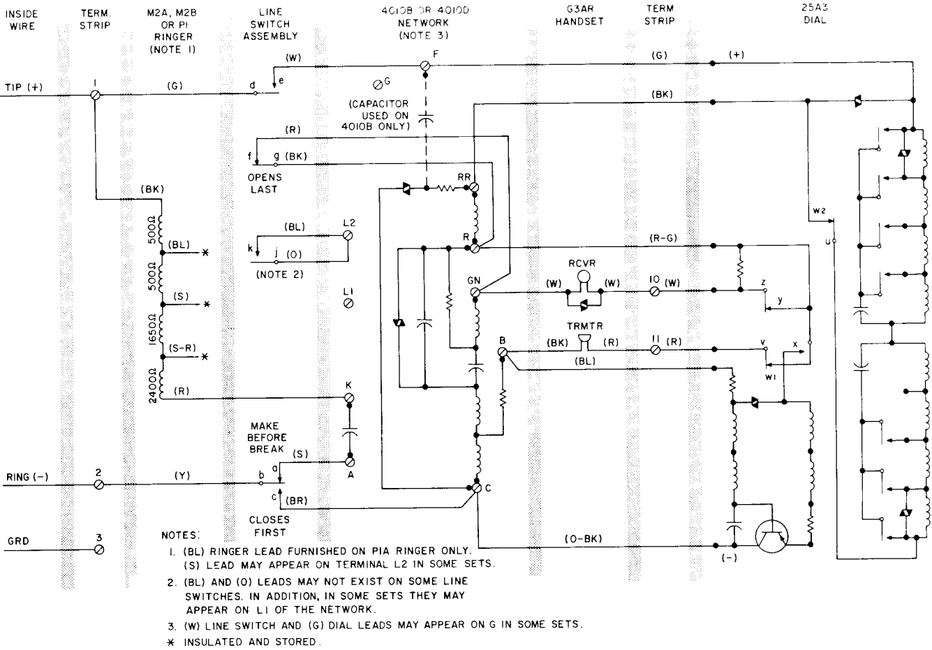
Fig. 1 — 1554B Telephone Set Connections, With 25A3 Dial
