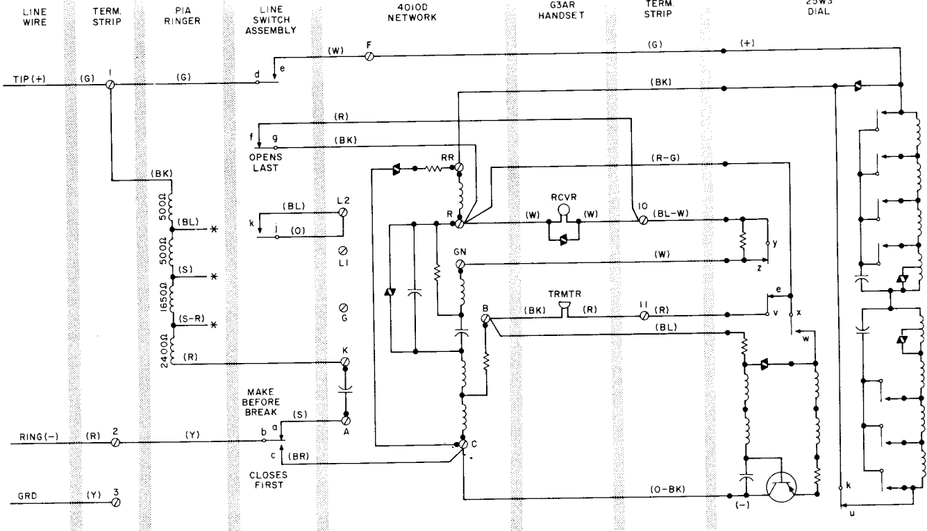
Fig. 1 — 1554B Telephone Set Connections, With 25A3 Dial
