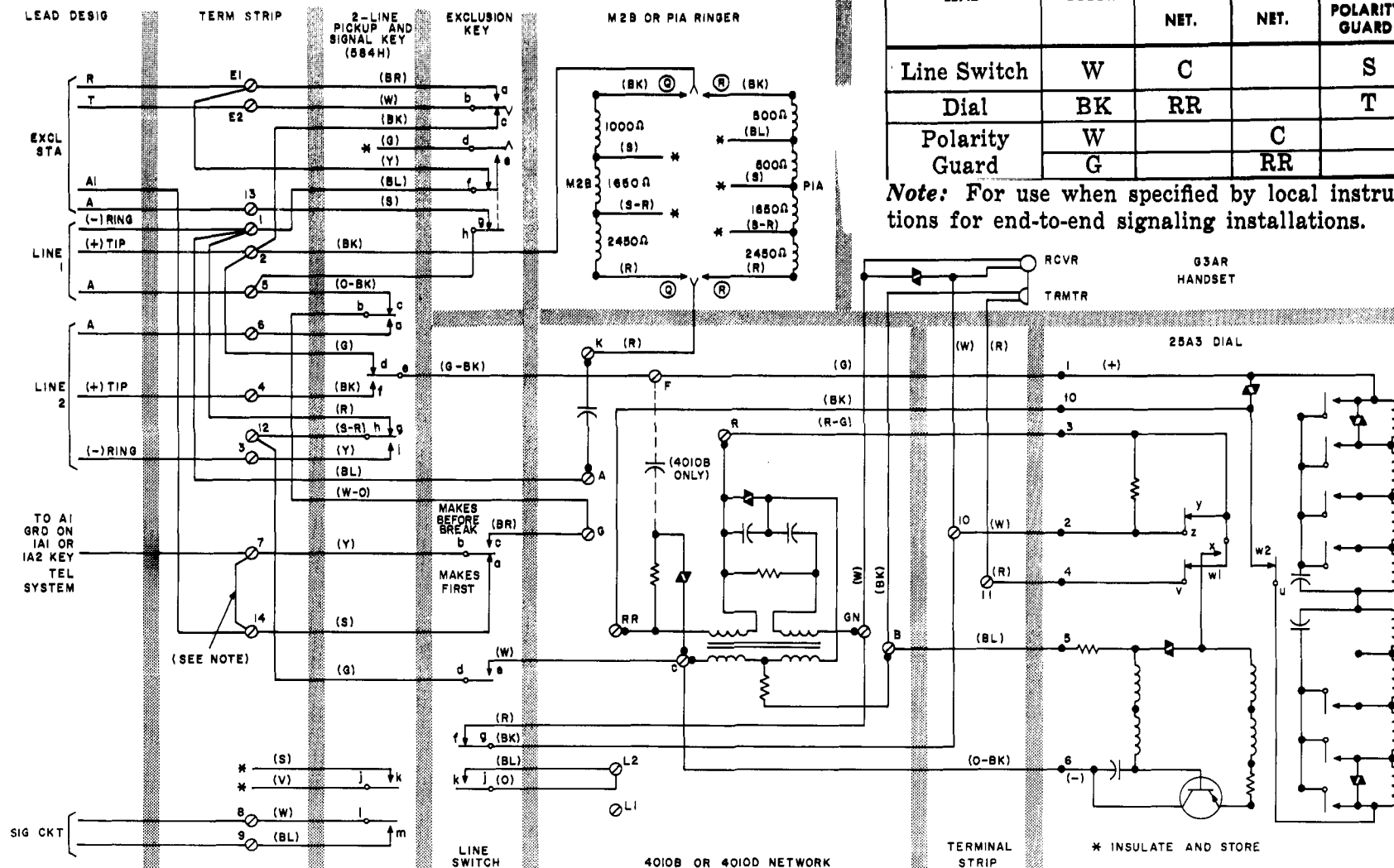
Fig. 1 — 2-Line Pickup With Exclusion on Line 1, Signaling, Wired for 1A1 and 1A2 Key Telephone Systems (With 25A3 Dial)
