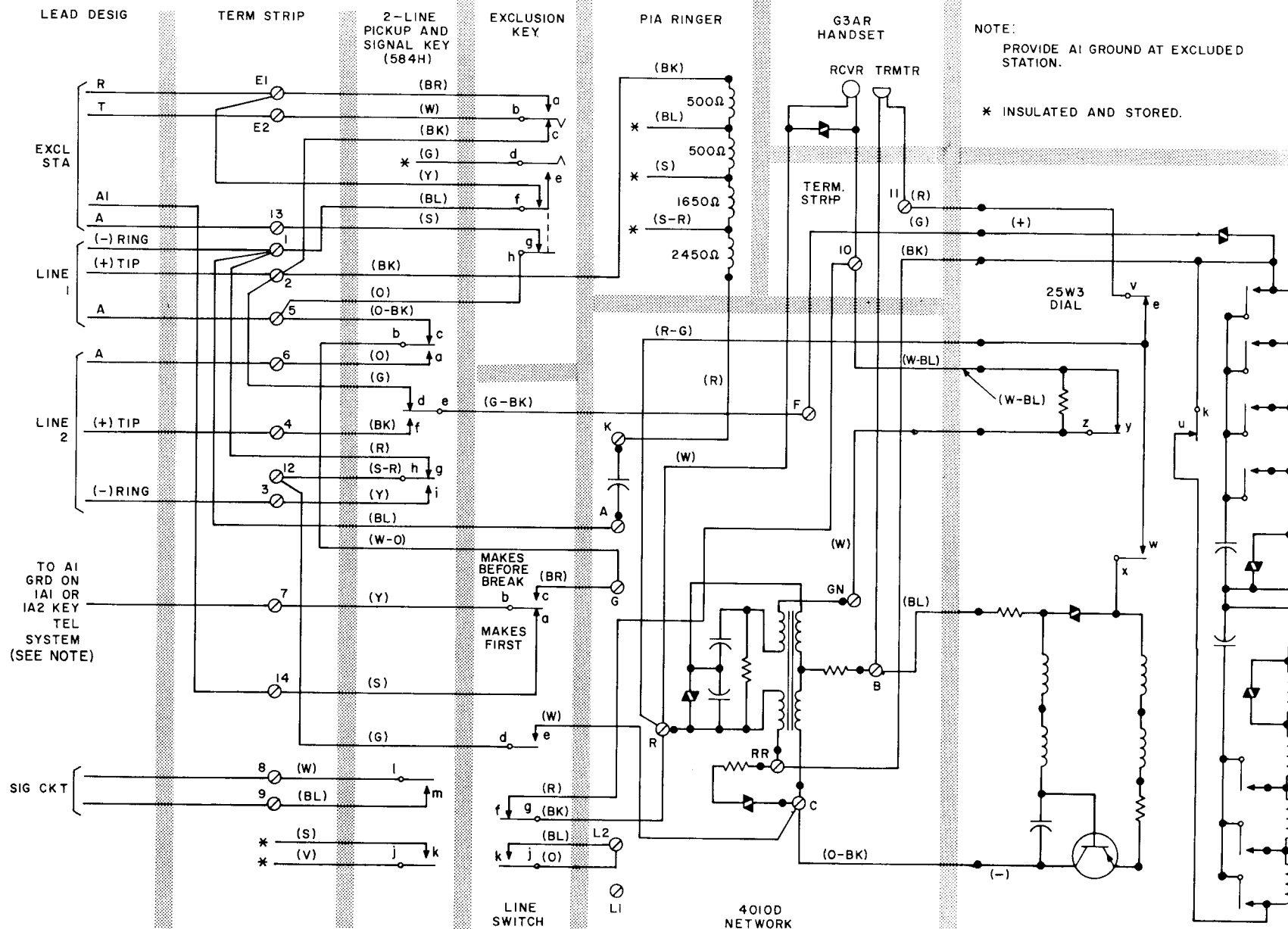
Fig. 2 — 2-Line Pickup With Exclusion on Line 1, Signaling, Wired for 1A1 and 1A2 Key Telephone Systems (With 25W3 Dial)
