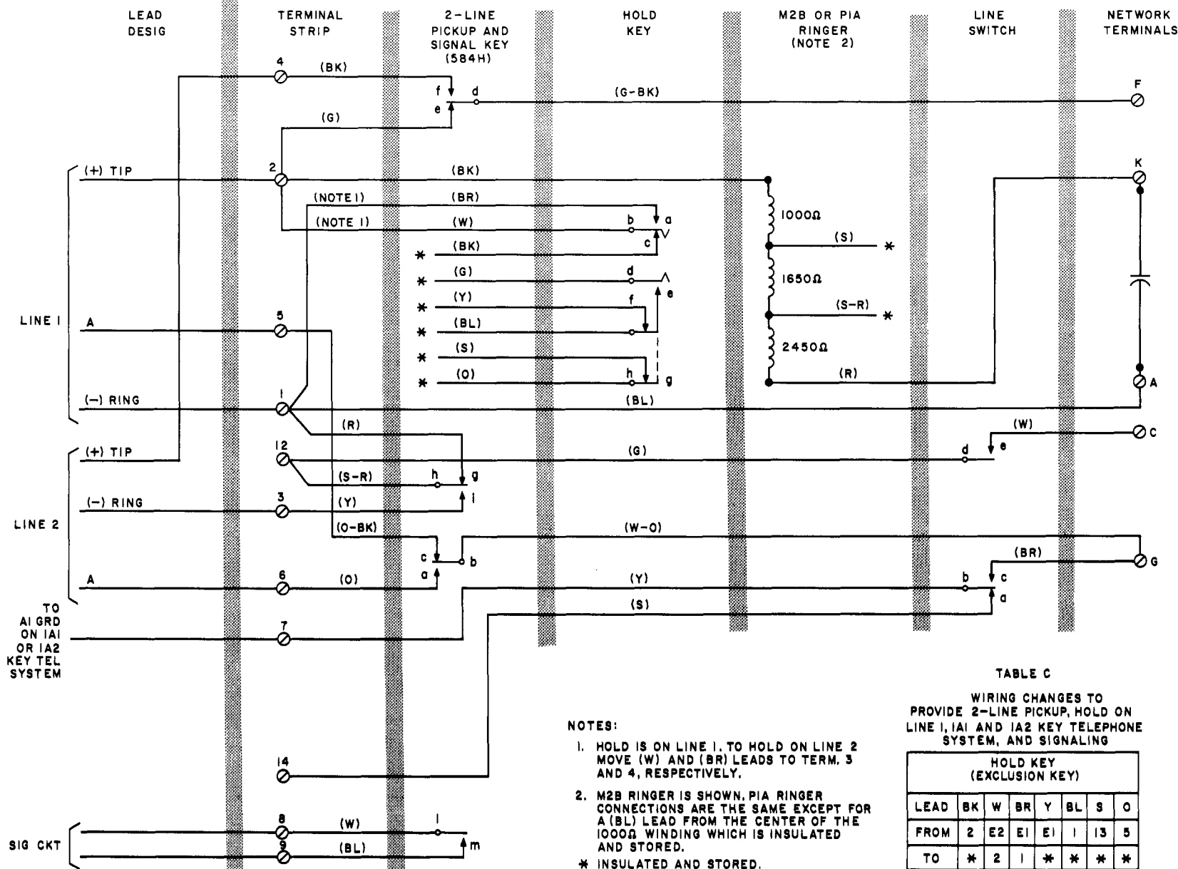
Fig. 4 — 2-Line Pickup, Hold on Line 1, Used With 1A1 and 1A2 Key Telephone Systems and Signaling
