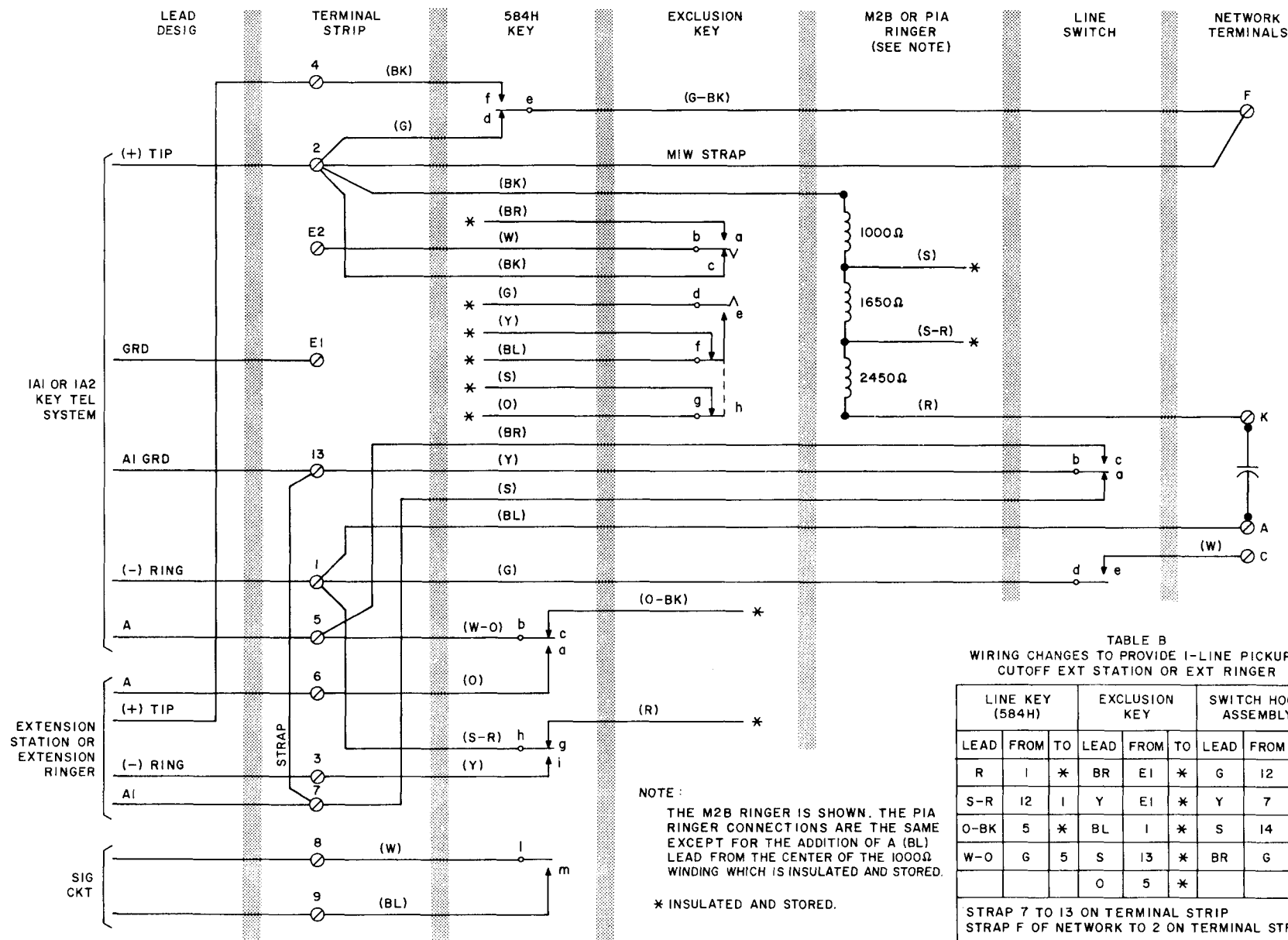
Fig. 3 — 1-Line Pickup, Cutoff Extension Station or Extension Line Ringer
