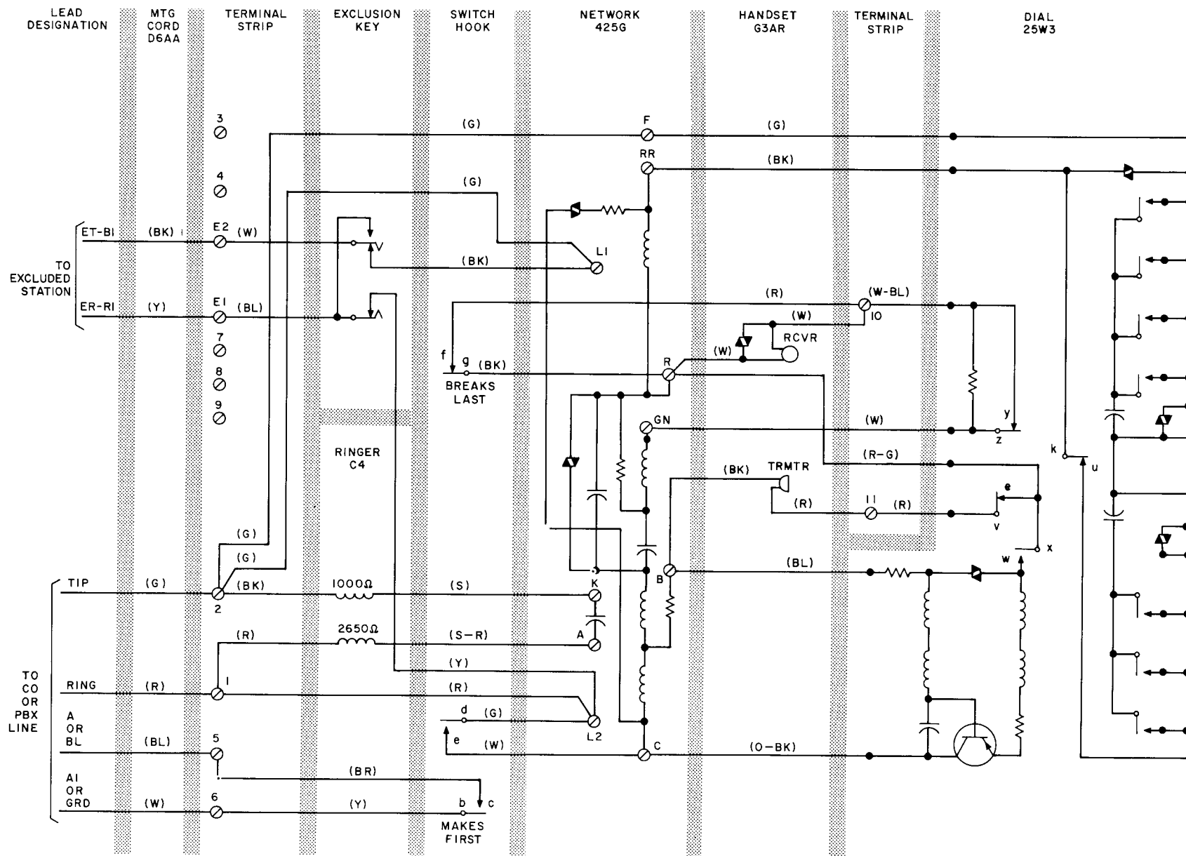
Fig. 2 — 1502B Telephone Set With 25W3 Dial
