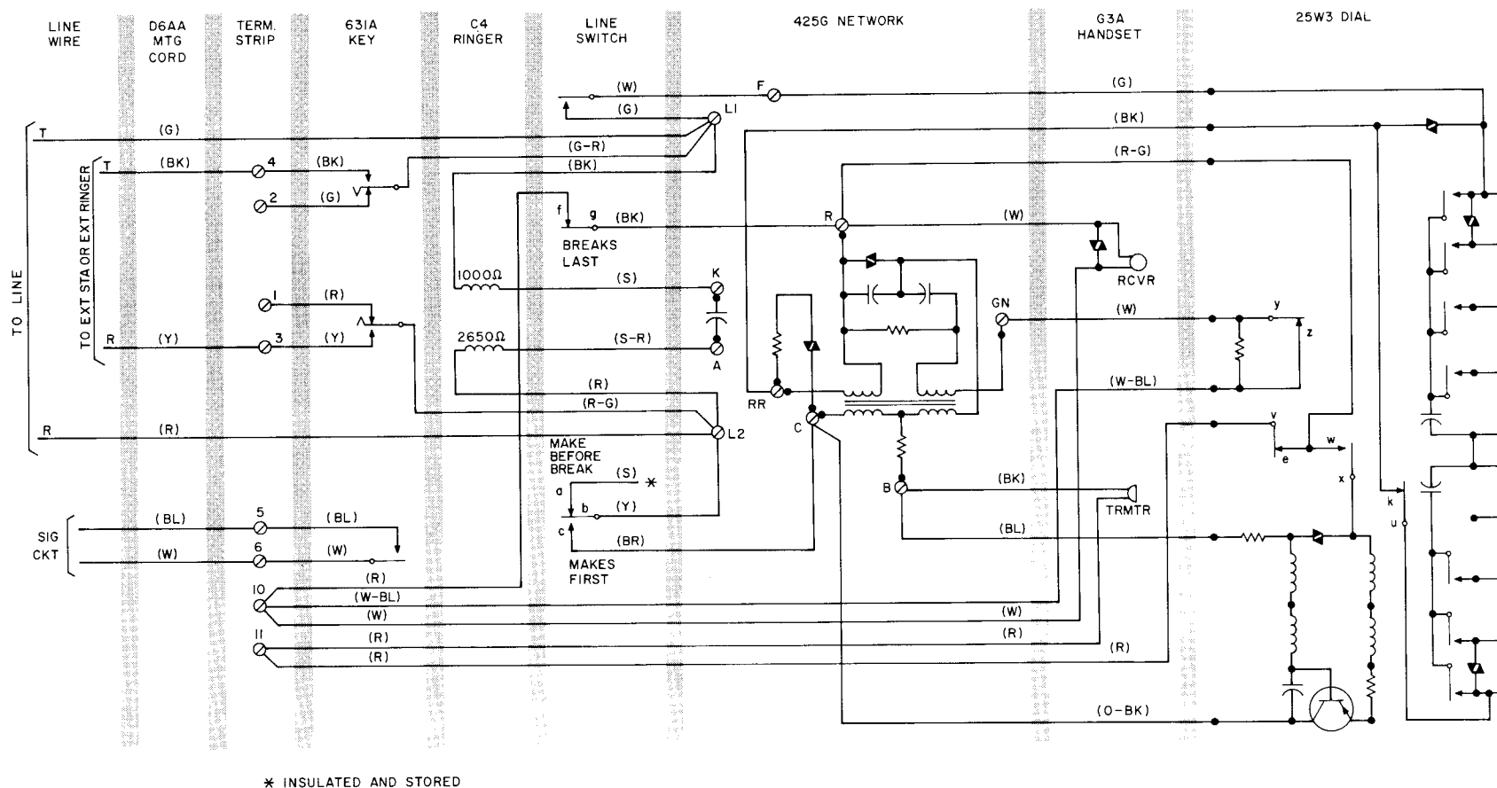
Fig. 4—1510F Telephone Set, With 25W3 Dial, Line Pickup, Cutoff of Extension Station or Ringer and Signaling
