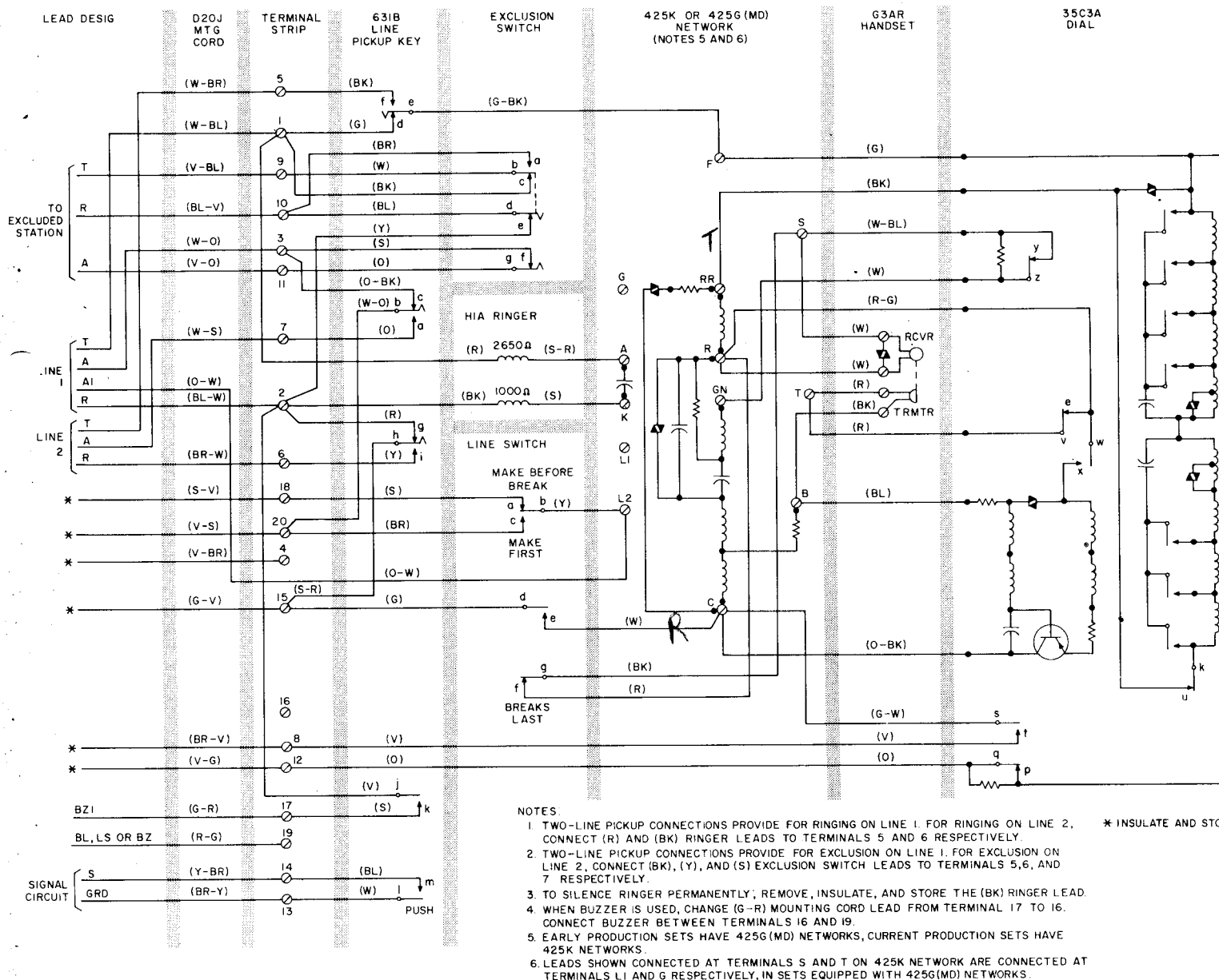
Fig. 2—2511F Telephone Set Connections, 2-Line Pickup With Exclusion on Line 1, Signaling Wired for 1A1 and 1A2 Key Telephone Systems
