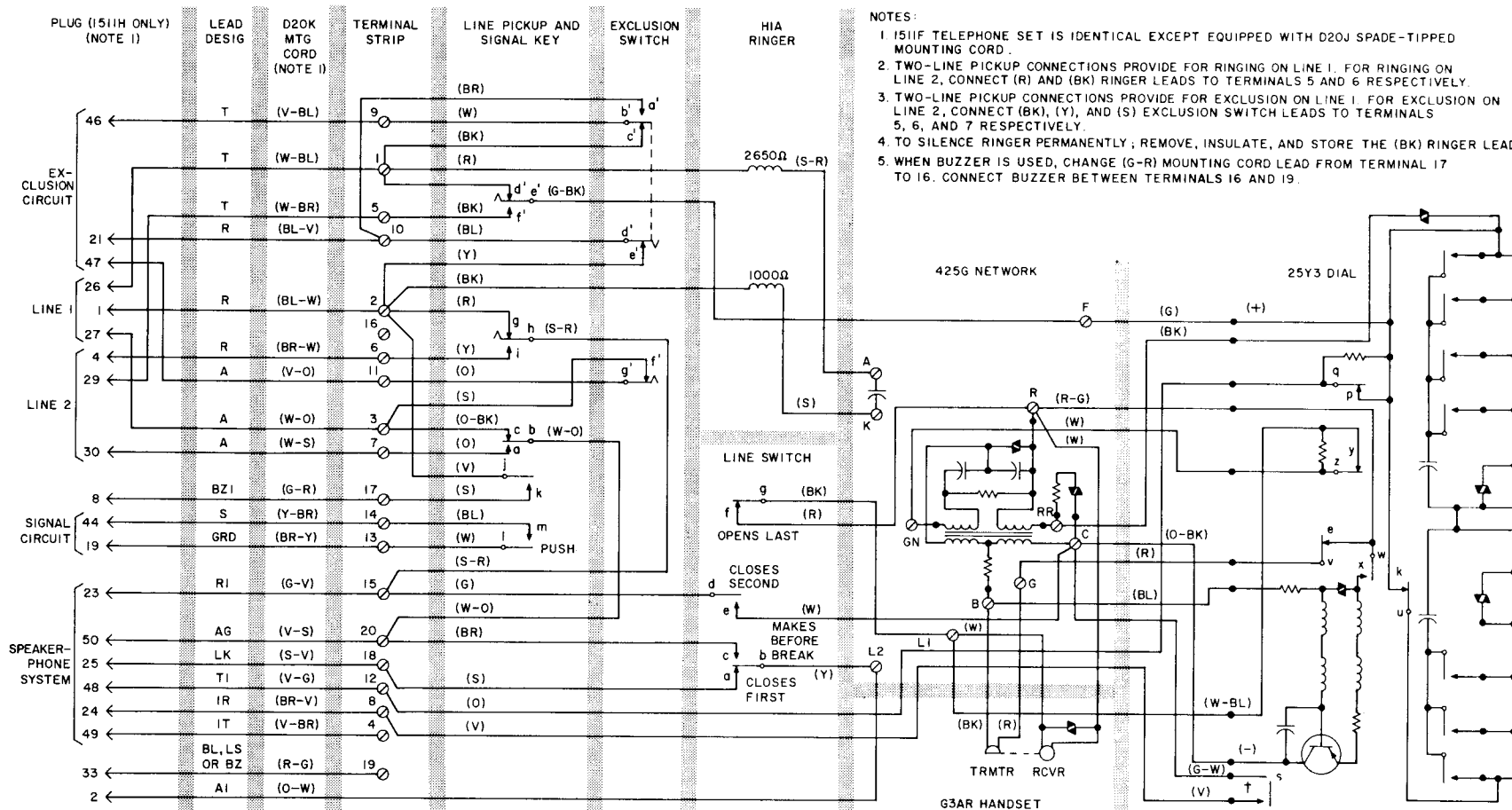
Fig. 3 — 1511F/H — 2-Line Pickup With Exclusion on Line 1, Signaling, and Speakerphone (Factory Wired With 25Y3 Dial)
