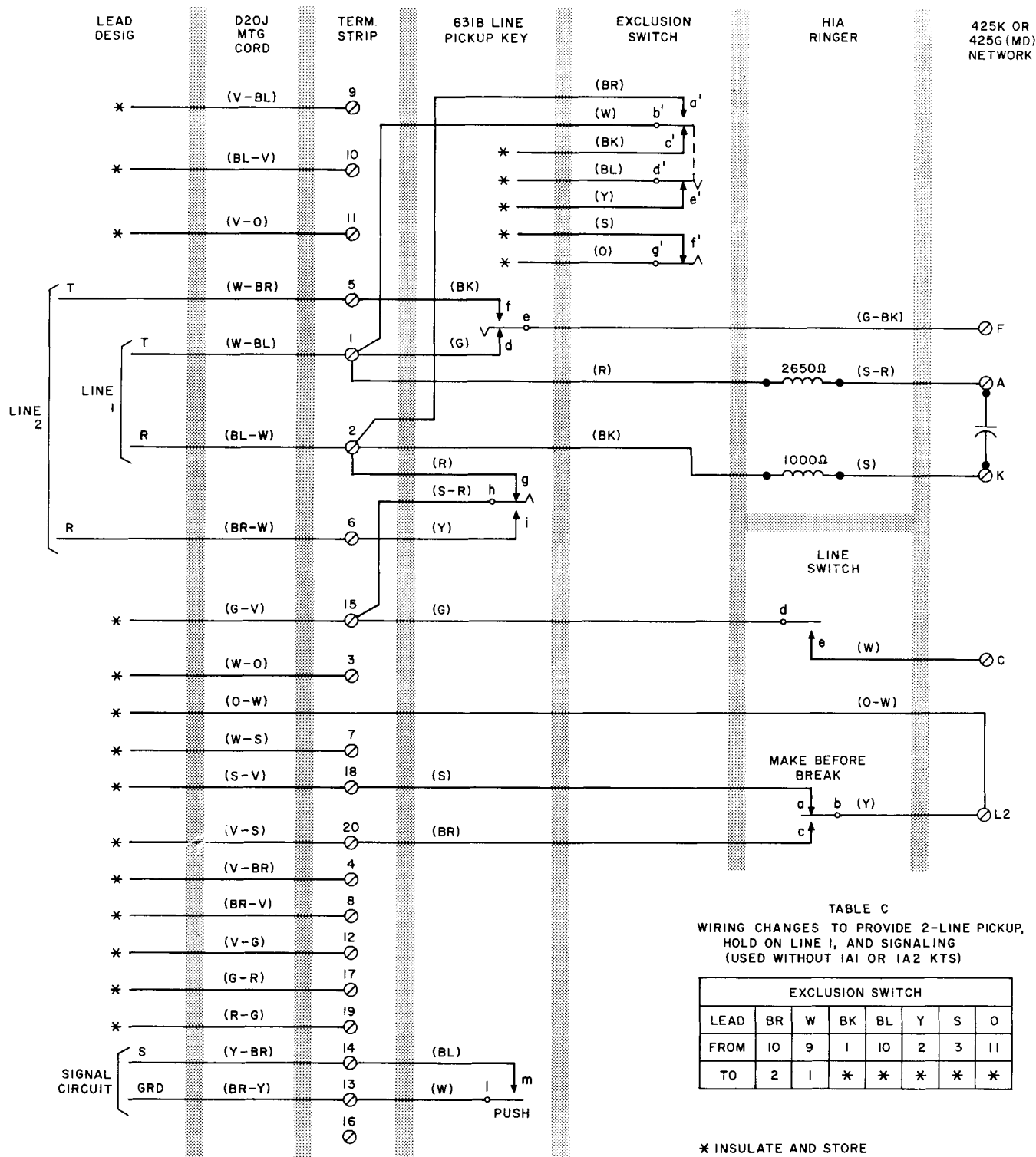
Fig. 4—2511F Telephone Set Connections, 2-Line Pickup, Hold on Line 1, and Signaling (Used Without 1A1 or 1A2 KTS)
