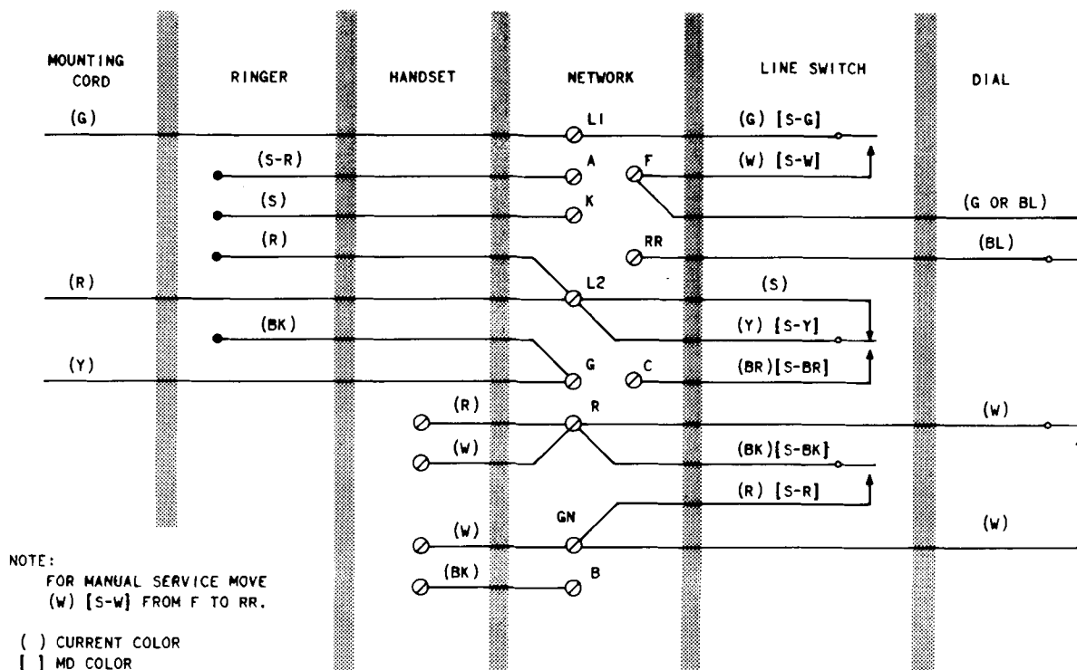
Fig. 1—500C/D Telephone Set, Connections
