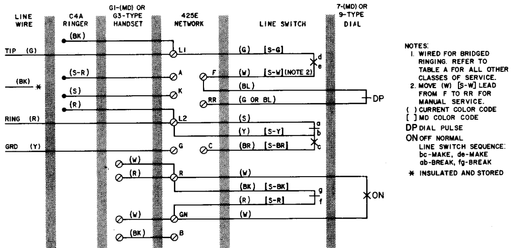
Fig. 1—554A/B and F Telephone Sets, Connections
