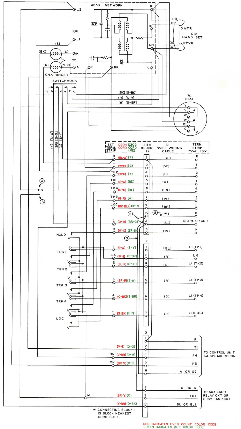
Fig. 6 — 566MB Telephone Set Used with 755A Dial PBX
