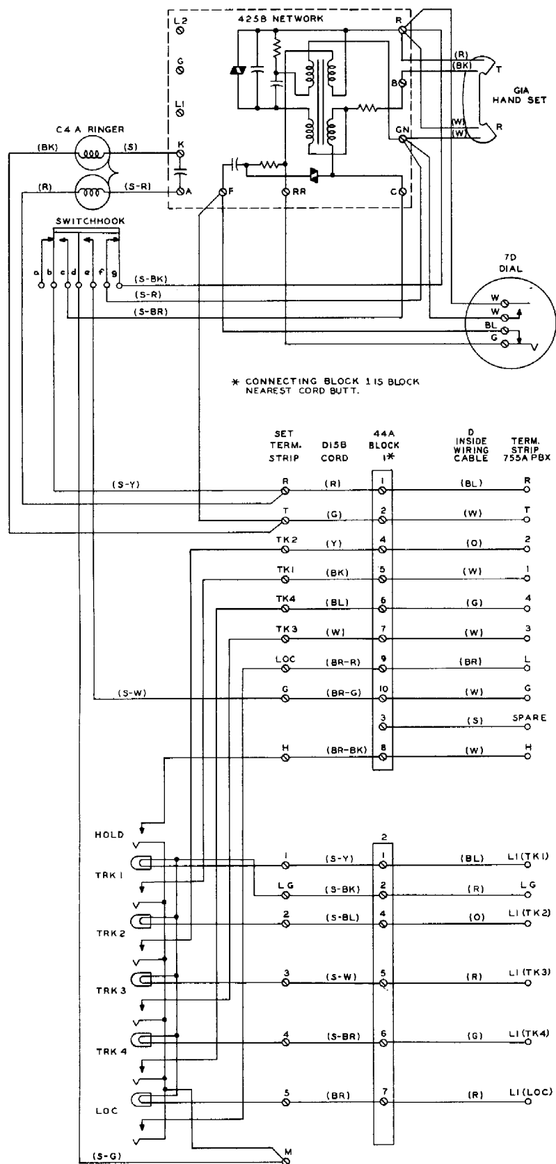
Fig. 5 — 566FB Telephone Set Used with 755A Dial PBX
