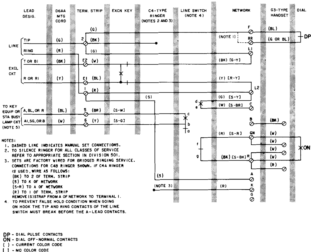
Fig. 1—502A/B Telephone Set, Connections
