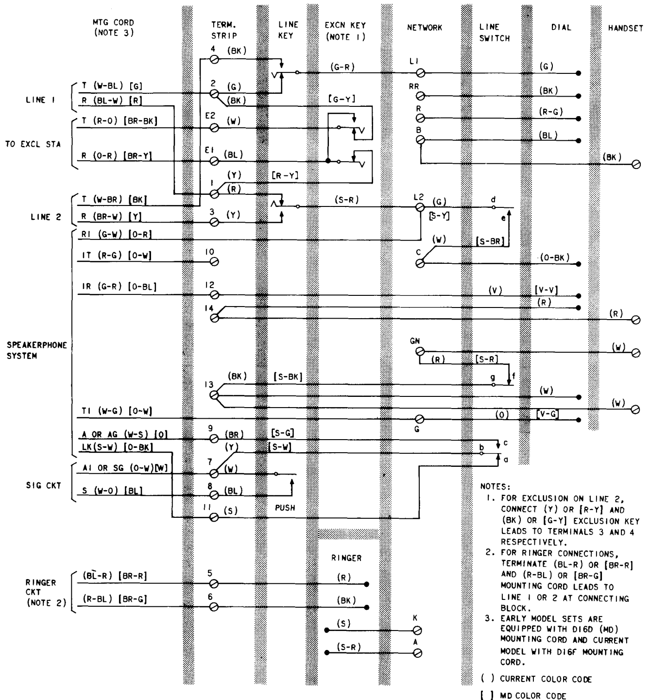
Fig. 2—1511D (MD) Telephone Set Connections, Equipped With 25B3 (MD) Dial
