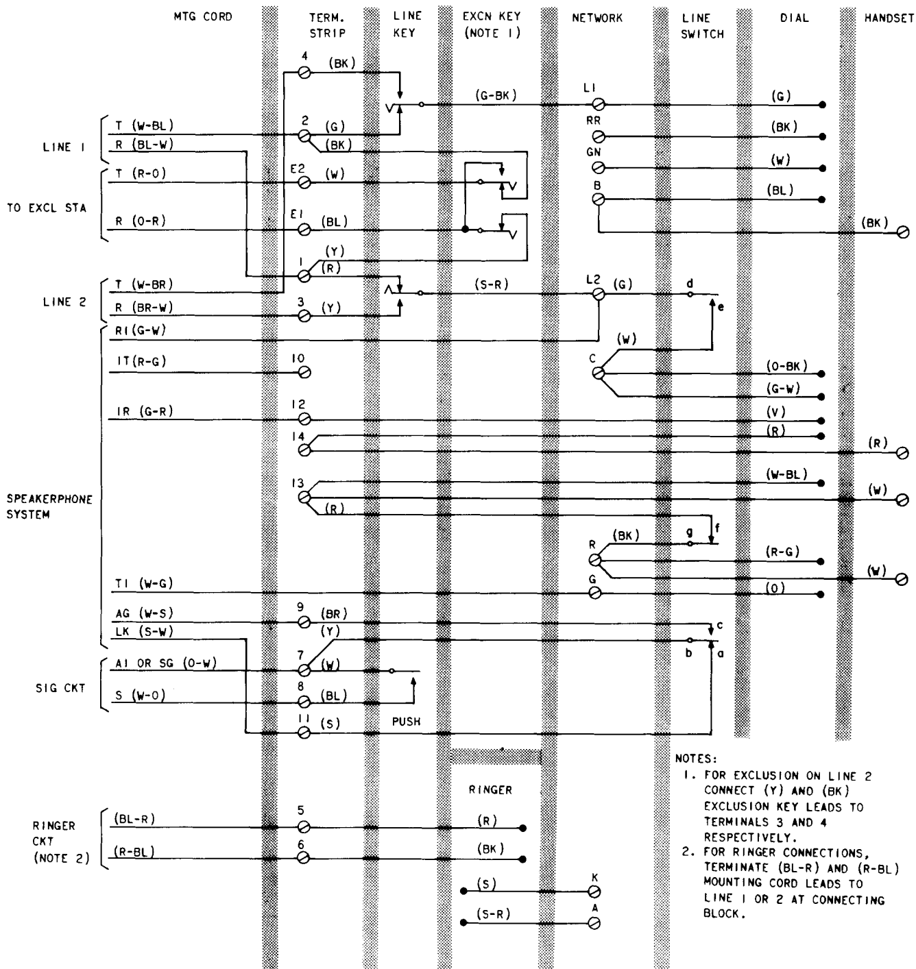
Fig. 1—1511D (MD) Telephone Set Connections, Equipped With 25Y3 Dial
