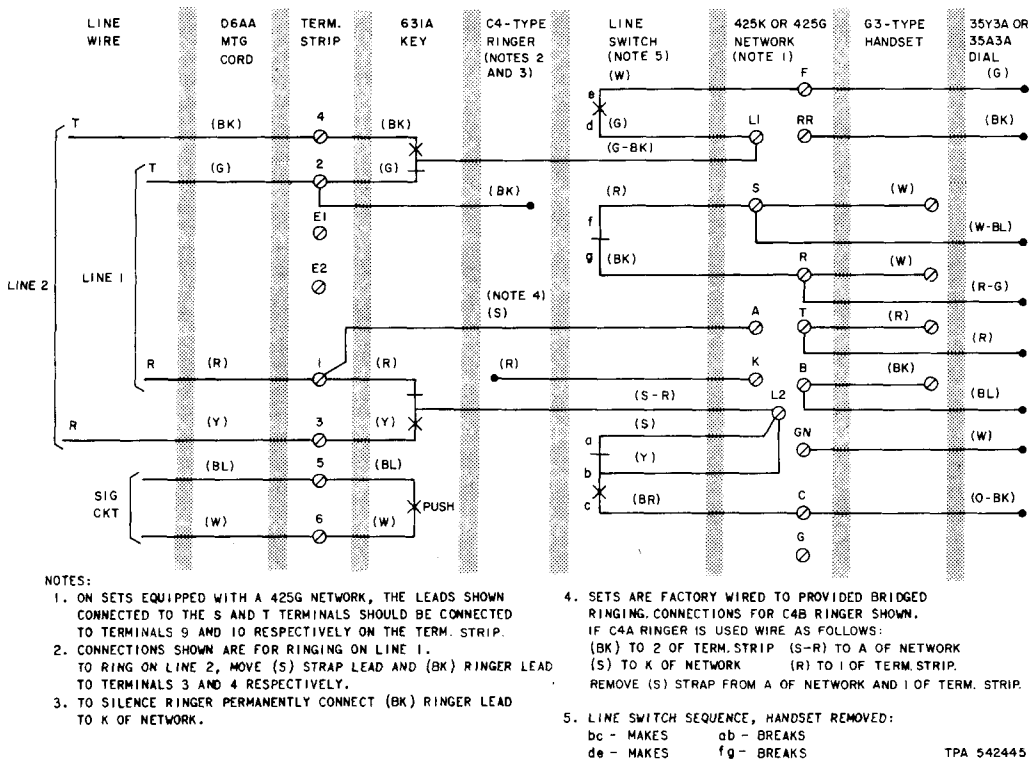
⚡Fig. 1—2510F Telephone Set Connections, 2-Line Pickup and Signaling⚡
