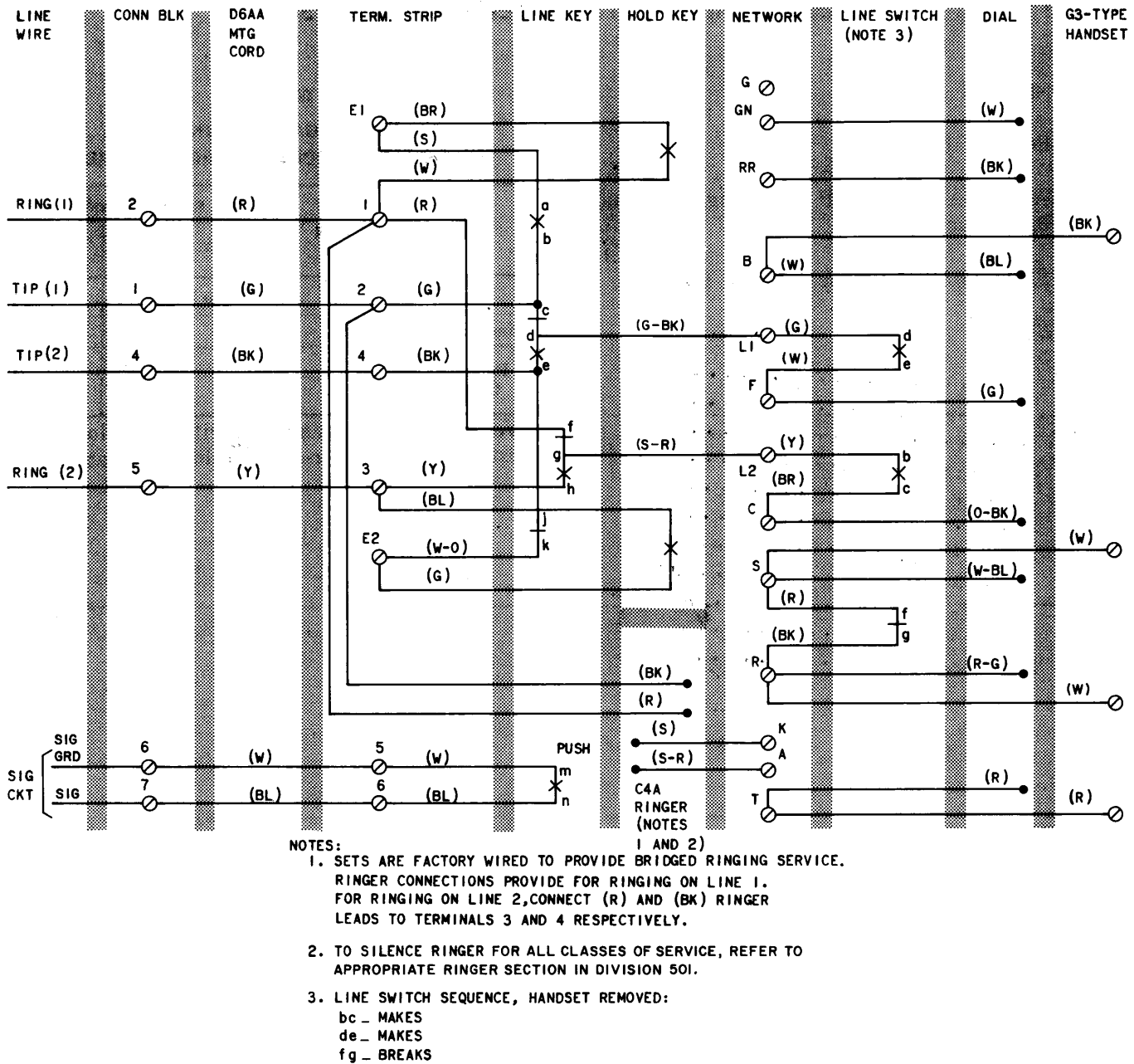
Fig. 1—2515B (MD) Telephone Set Connections, 2-Line Pickup, Hold, and Signaling (Factory Wired)
