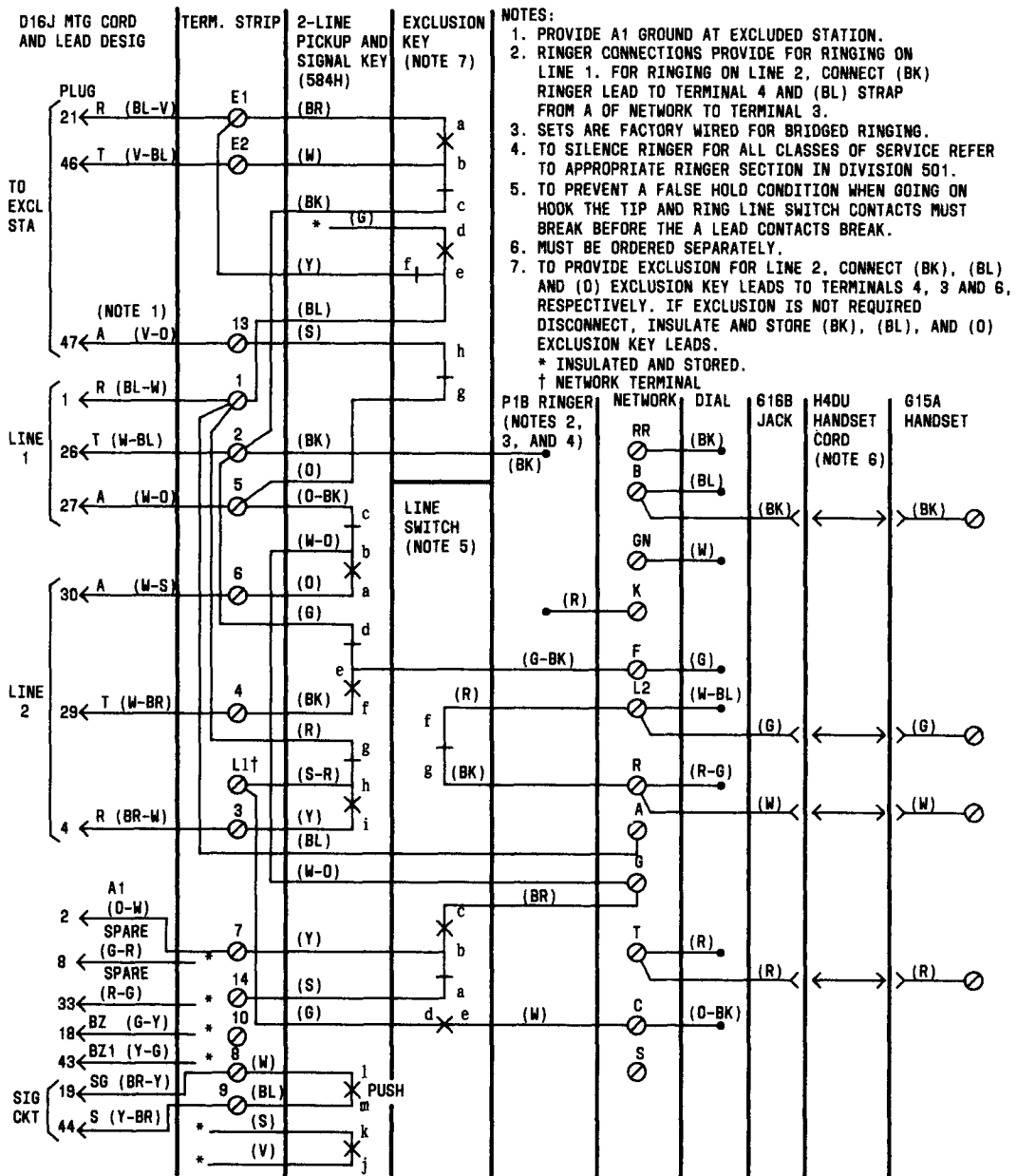
Fig. 2—2558DM Telephone Set, Connections (Factory Wired)
