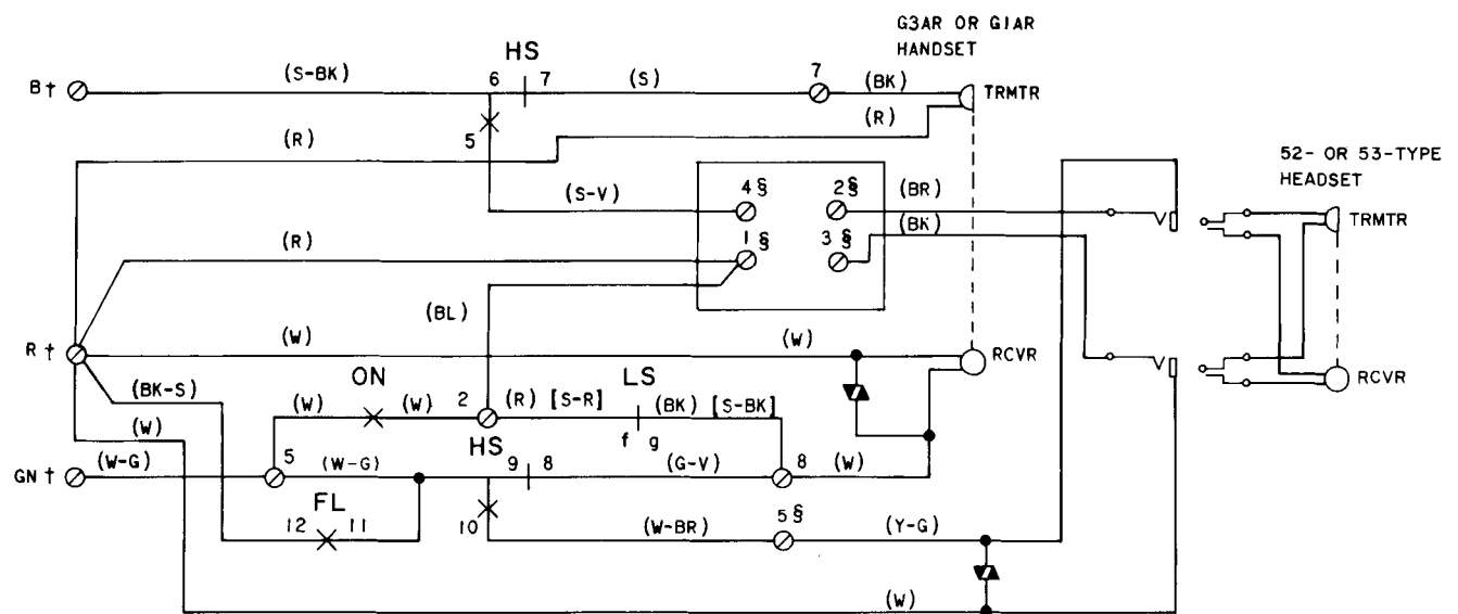
241A AMPLIFIER SERIES II (NOTE 10)
