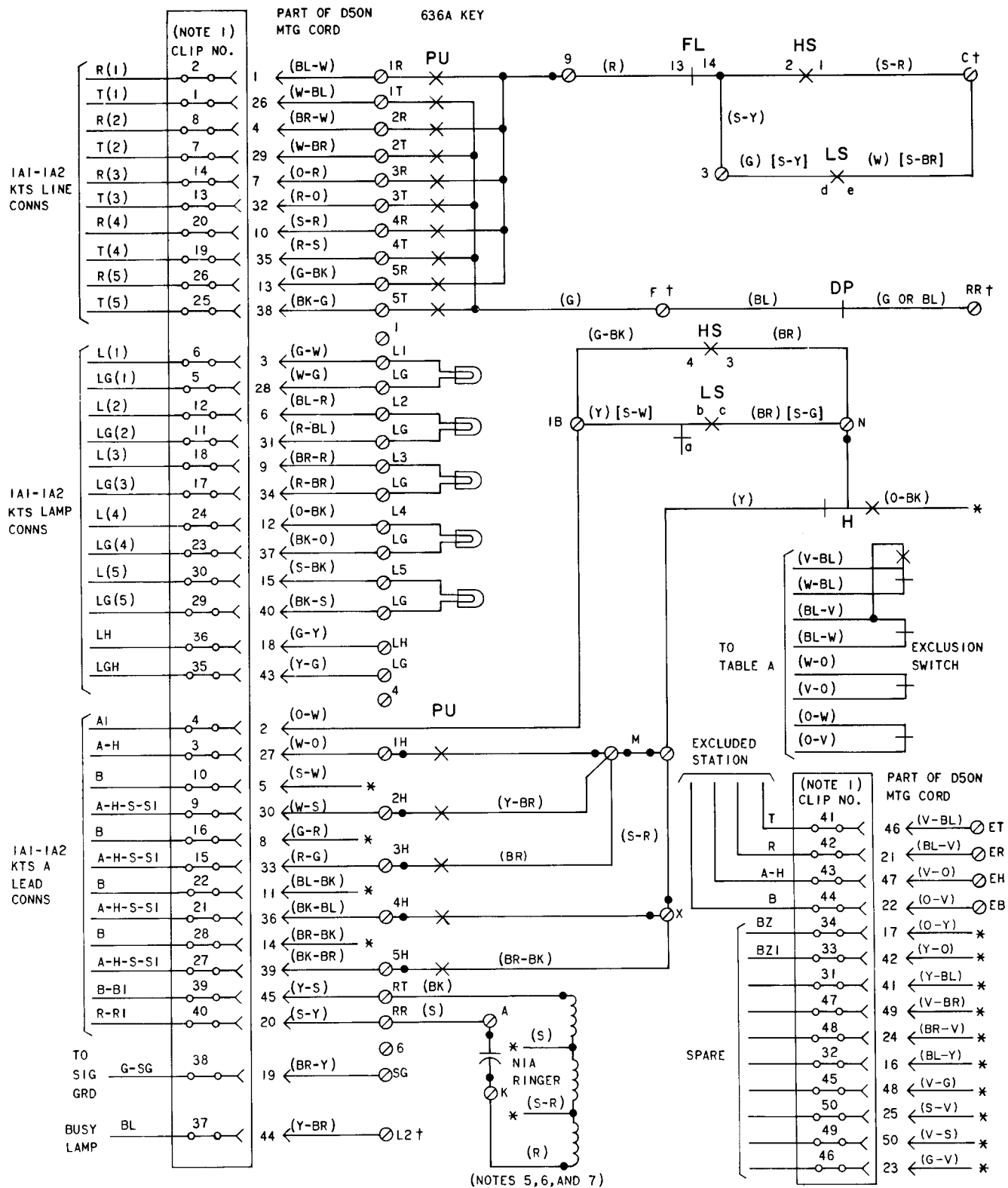
Fig. 1—563HB Telephone Set, Connections (Sheet 1 of 2)
