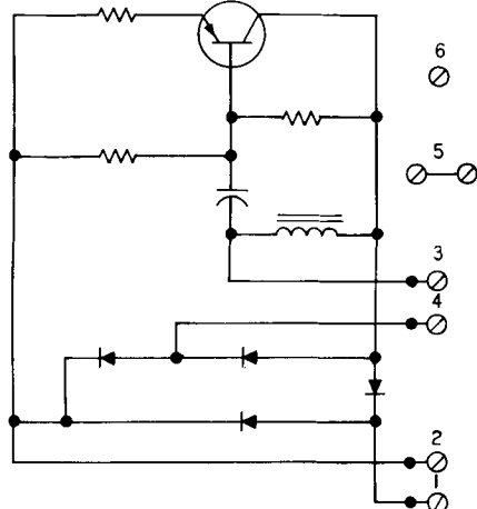
241A AMPLIFIER SERIES II (NOTE 10)
