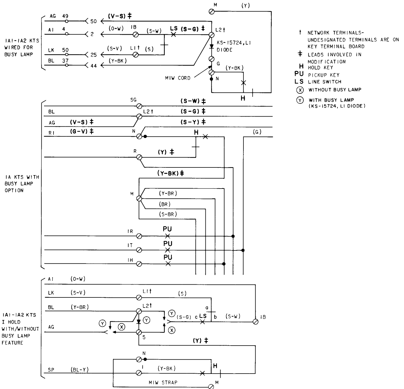
Fig. 6—Optional Features for 565HDR (MD) Telephone Set
