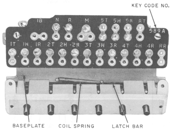
Fig. 3—589-Type Key, Top View
