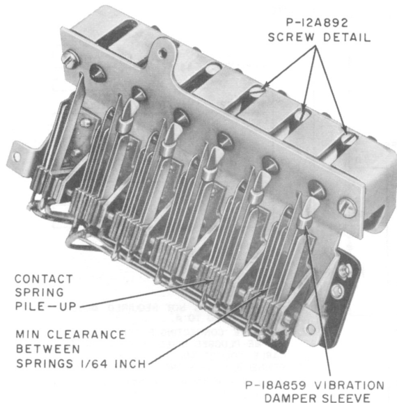
Fig. 4—589-Type Key, Bottom View
