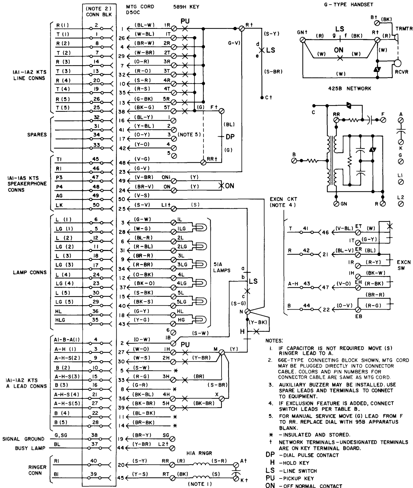
Fig. 5-565HDR (MD) Telephone Set
