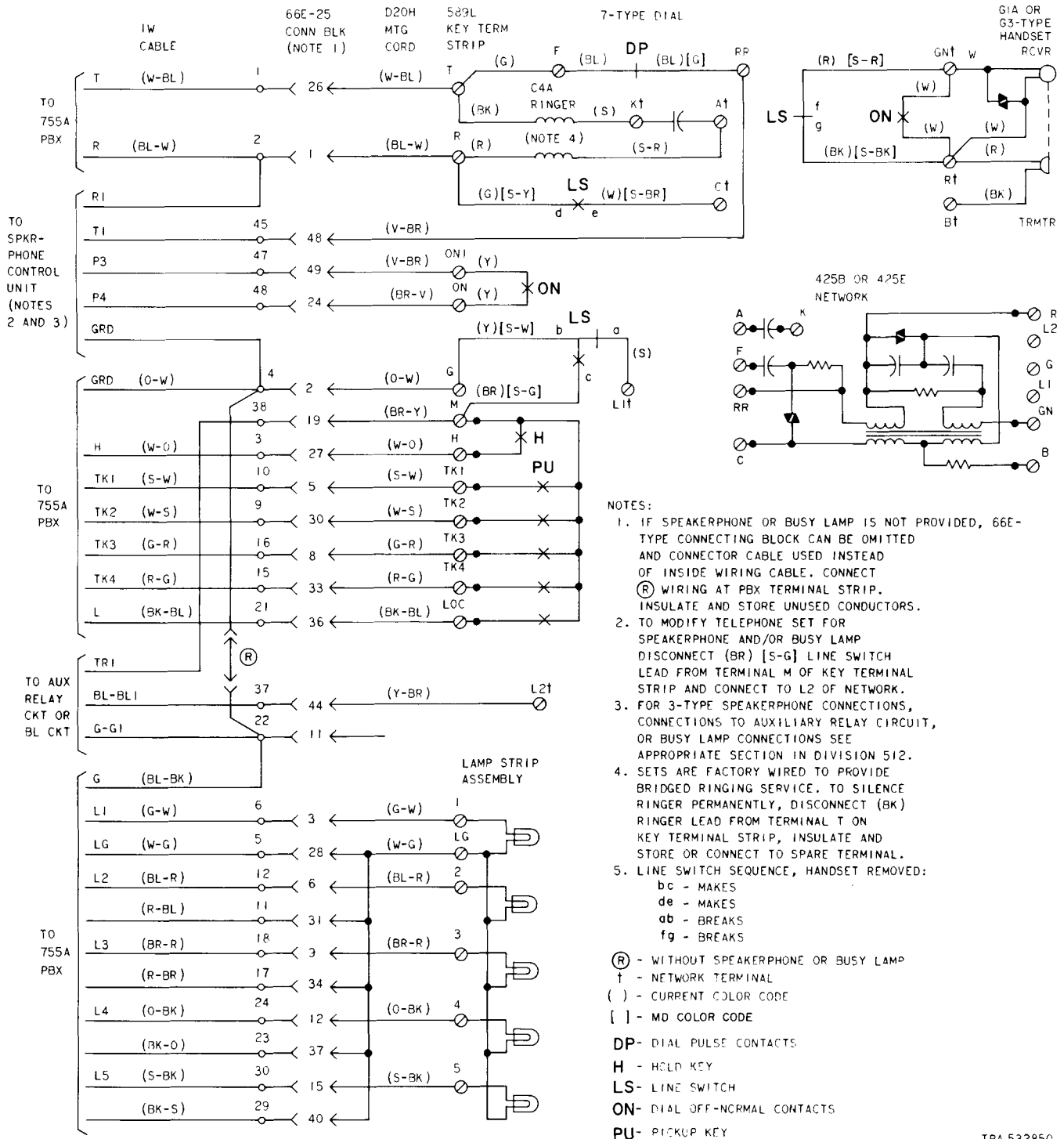
Fig. 2—566MB (MD) Telephone Set Connections to 755A PBX Using 66E Type Connecting Block, With Speakerphone and/or Busy Lamp
