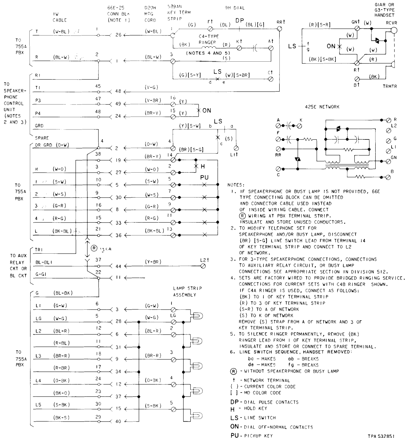
Fig. 1—566MD Telephone Set Connections to 755A PBX Using 66E Type Connecting Block, With Speakerphone and/or Busy Lamp
