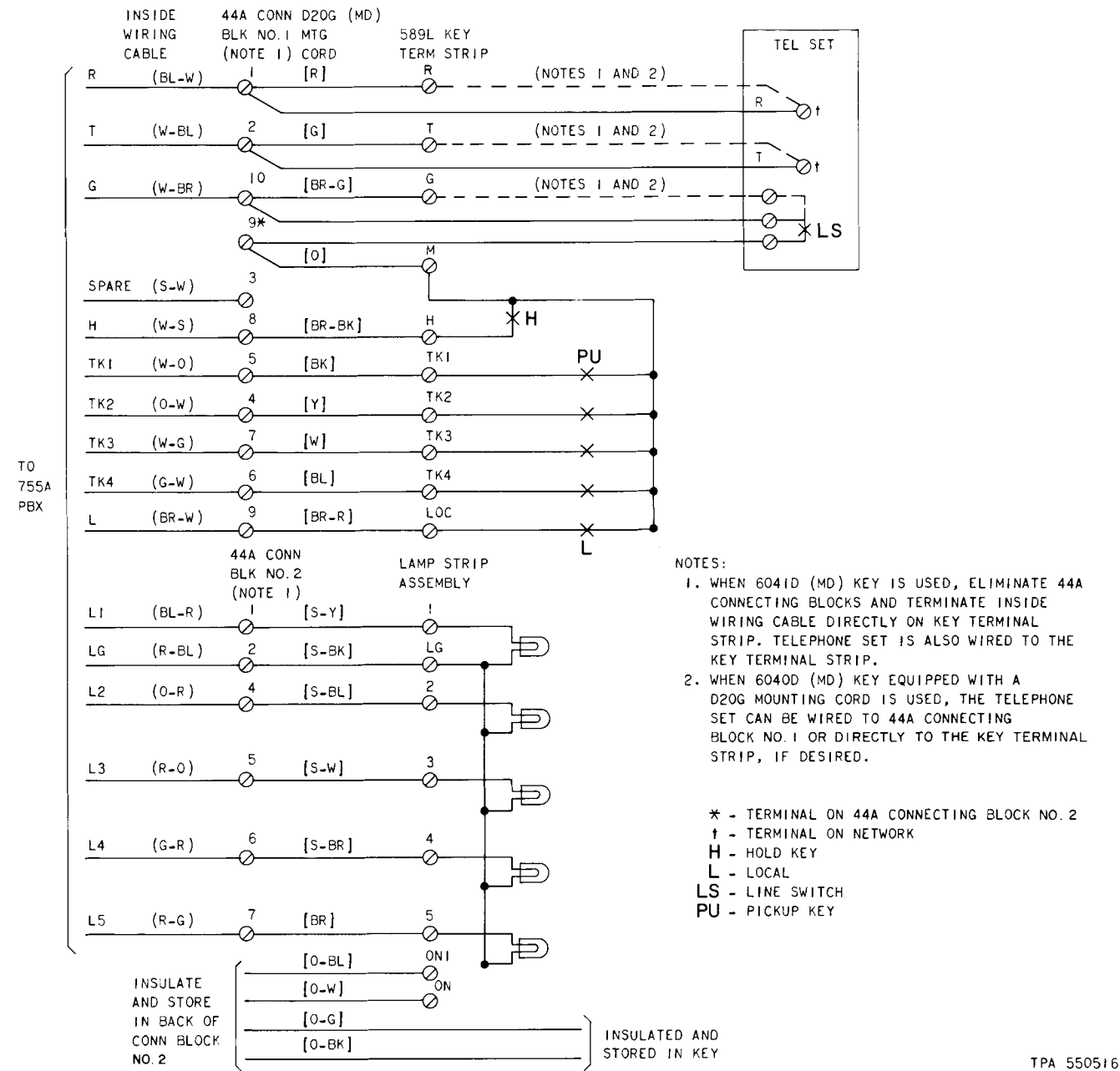
Fig. 5—6040D (MD) and 6041D (MD) Key Connections to 755A PBX
