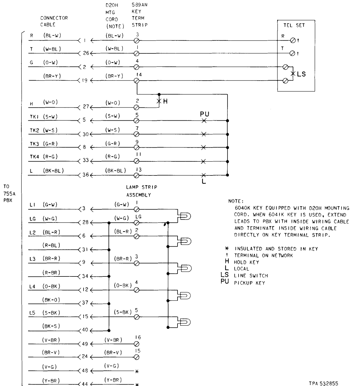
Fig. 4—6040K and 6041K Key Connections to 755A PBX
