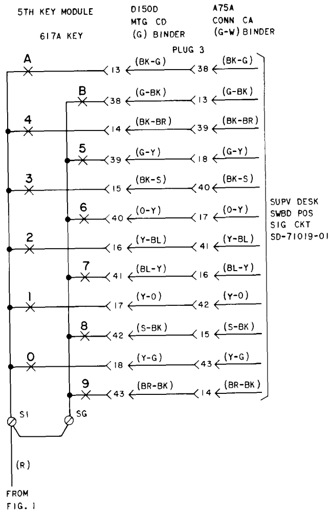
Fig. 2—Module and Mounting Cord Arrangement (Sheet 3 of 3)
