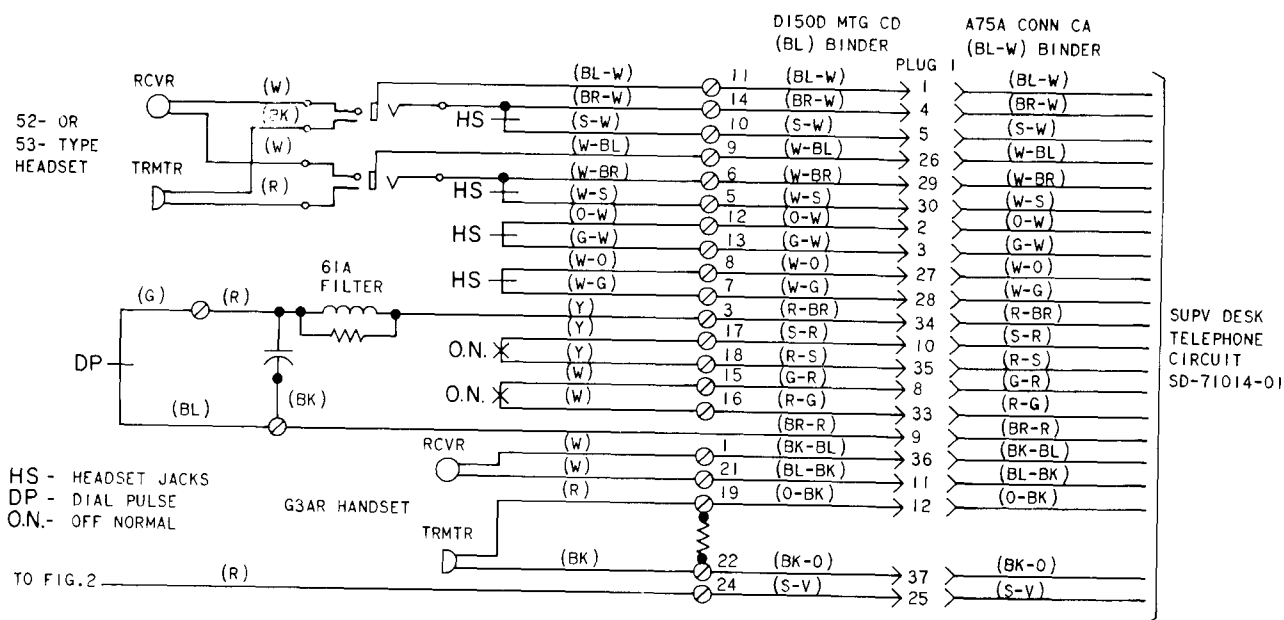
B. 609AI TELEPHONE SET
