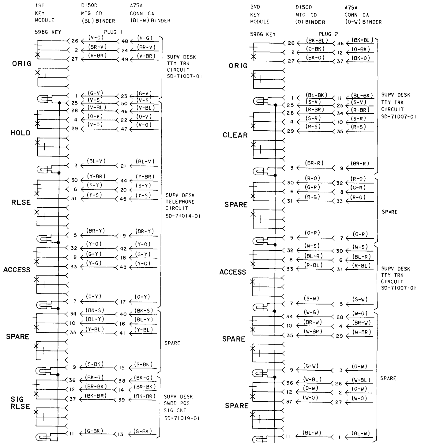
Fig. 2—Module and Mounting Cord Arrangements (Sheet 1 of 3)
