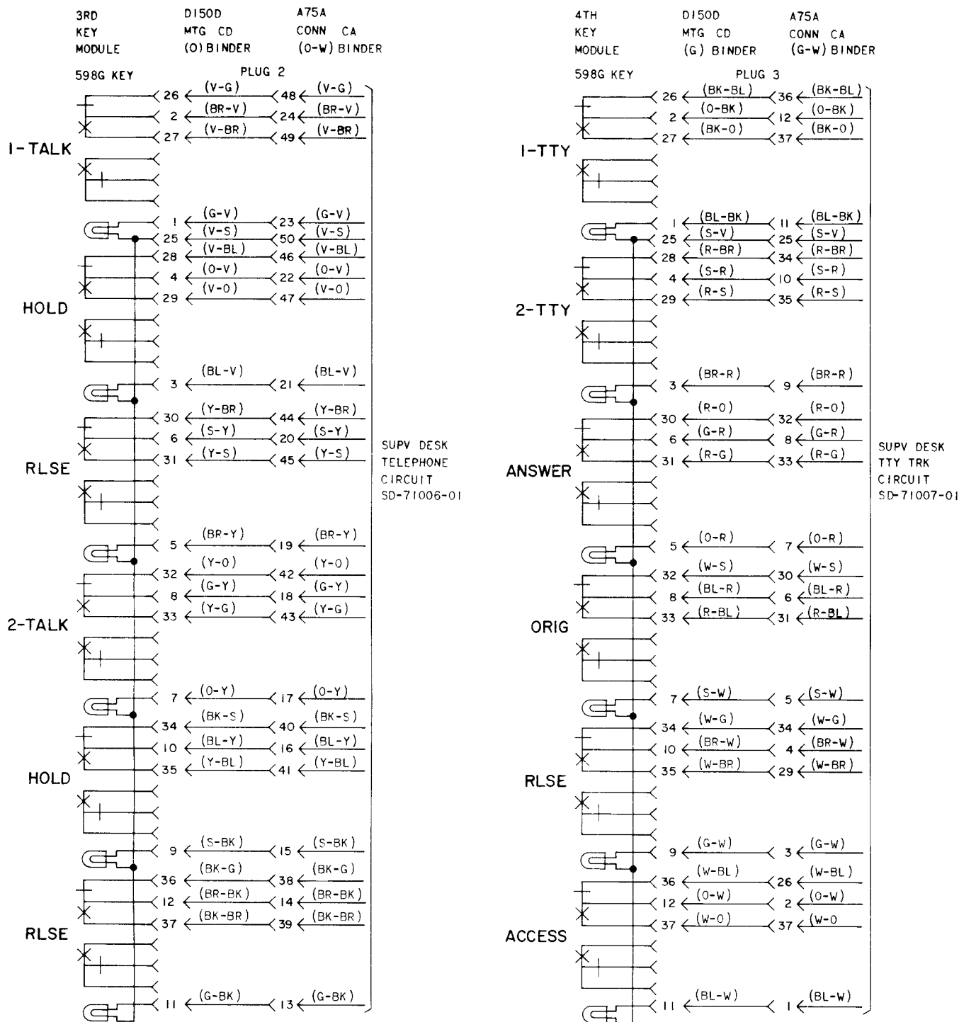
Fig. 2—Module and Mounting Cord Arrangements (Sheet 2 of 3)
